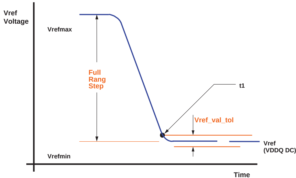
VREF Full Step From VREF,max to VREF,minCase
