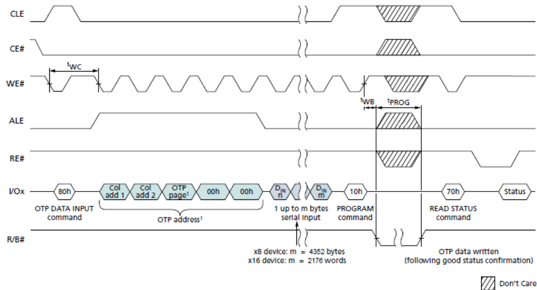
Figure 8.24 OTP Page Program (After Set Feature of OTP Operation Mode)
