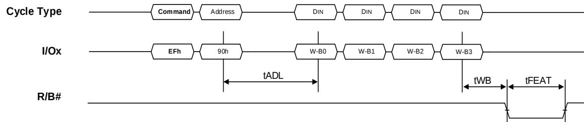
Figure 8.23 Set Features (EFh-90h) for OTP Mode Setting
