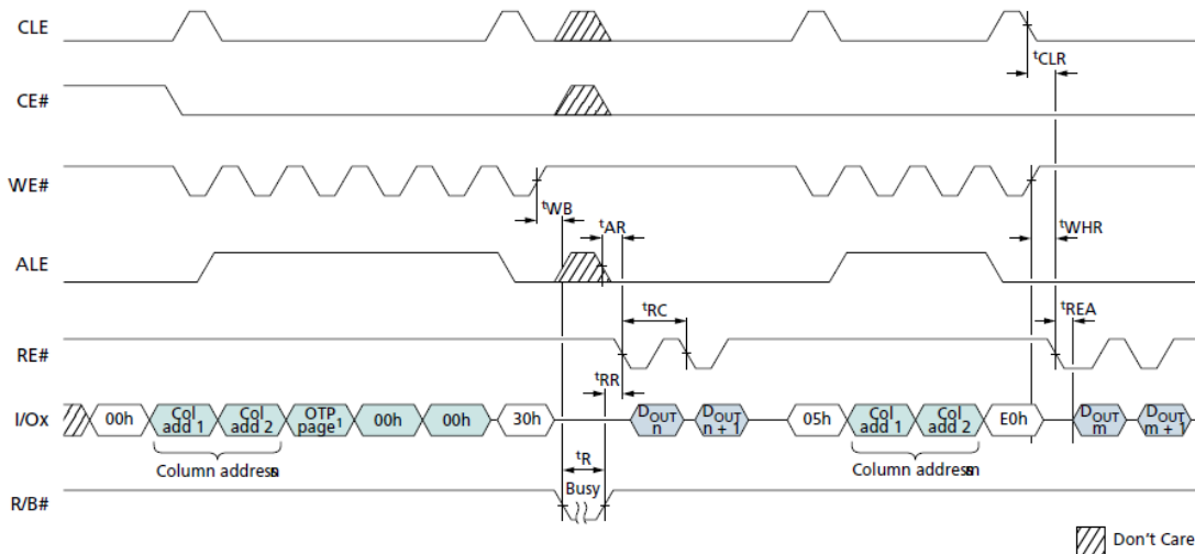
Figure 8.27 OTP Read with Random Data Output
