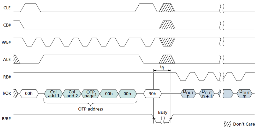
Figure 8.26 OTP Read
