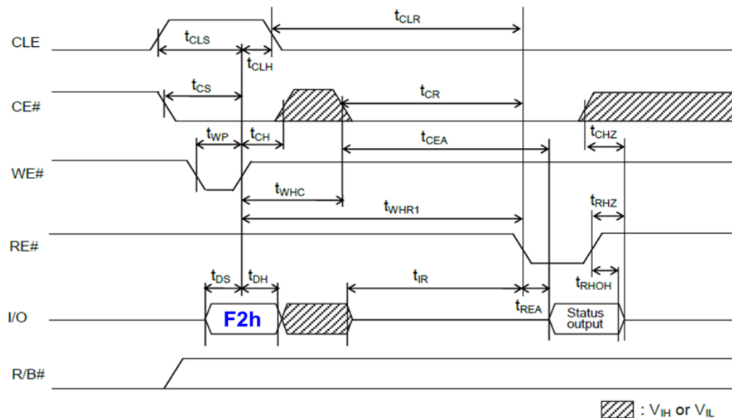
Figure 8.22 Die Selection Read Status Operation (F2h to select die 0).
