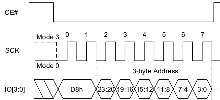
Figure 8.34 Block Erase (64K/256K) Sequence In QPI Mode (D8h [EXTADD=0], 3-byte address)
