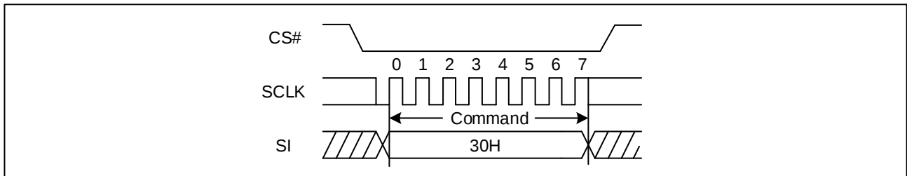
Figure 10. Clear Status Register Flags Diagram (SPI)
