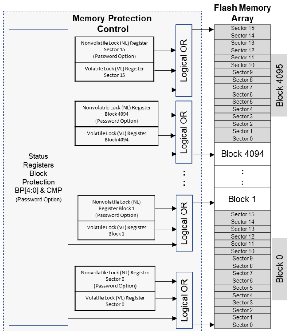
Figure 4 Memory Protection Control Overview
