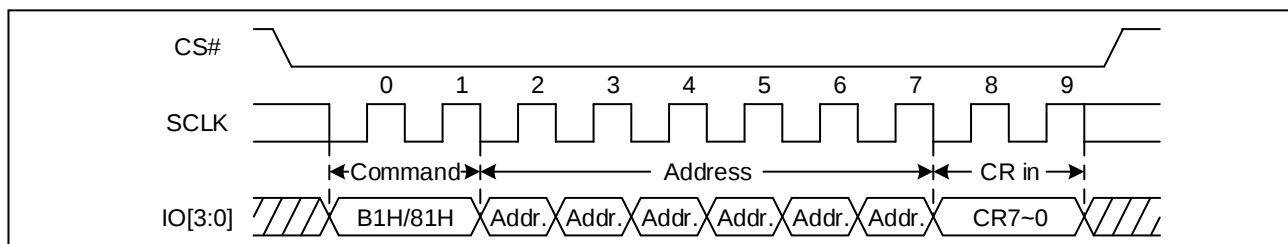
Figure 25 Write Nonvolatile/Volatile Configuration Register Sequence Diagram (QPI)
