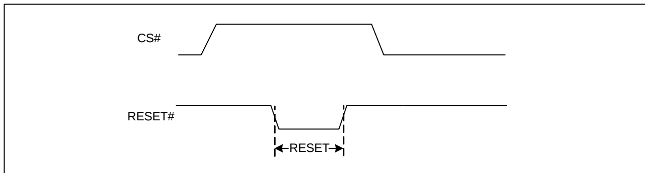
Figure 3 RESET Condition
