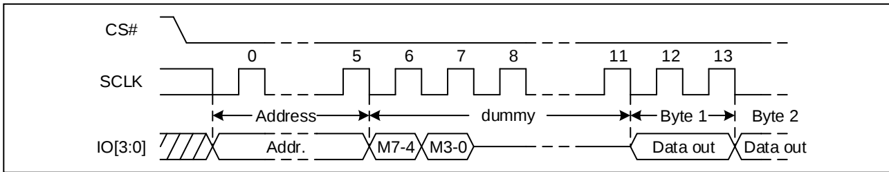
Figure 43 Quad I/O Fast Read Sequence Diagram (M5-4= (1, 0))
