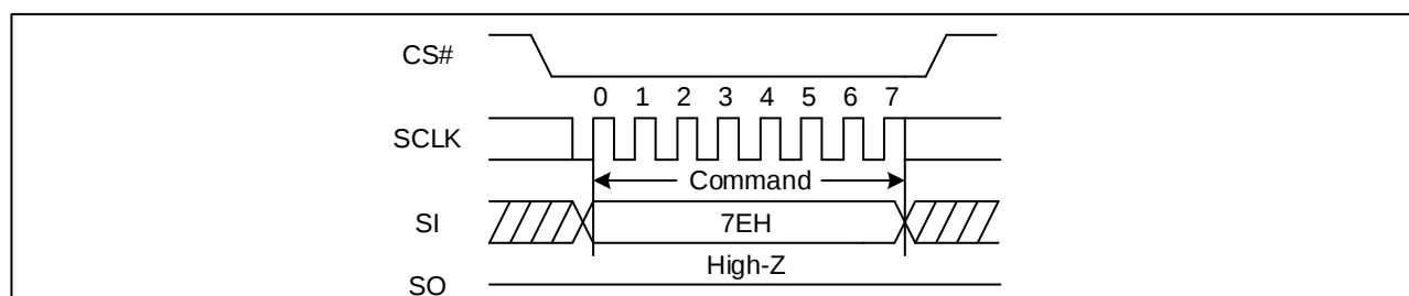
Figure 78 Global Block/Sector Lock Sequence Diagram (SPI)
