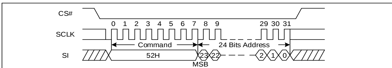
Figure 52 32KB Block Erase Sequence Diagram (SPI)
