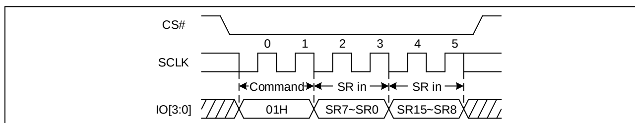
Figure 21. Write Status Register-1&2 Sequence Diagram (QPI)
