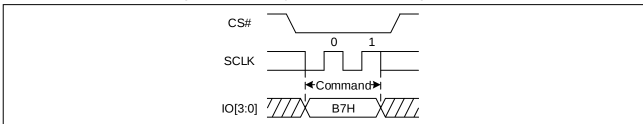
Figure 7 Enable 4-Byte Mode Sequence Diagram (QPI)
