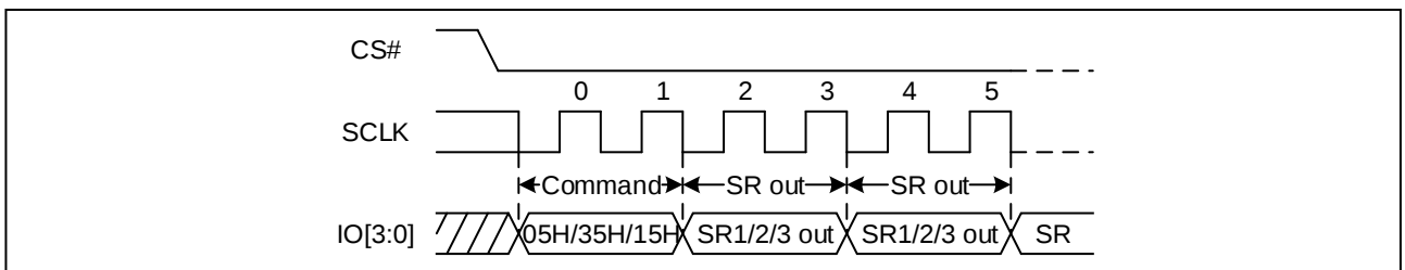
Figure 27 Read Status Register Sequence Diagram (QPI)
