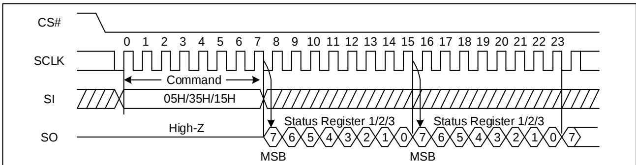
Figure 26 Read Status Register Sequence Diagram (SPI)
