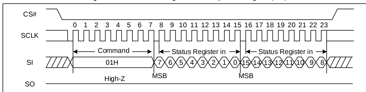
Figure 20. Write Status Register-1&2 Sequence Diagram (SPI)
