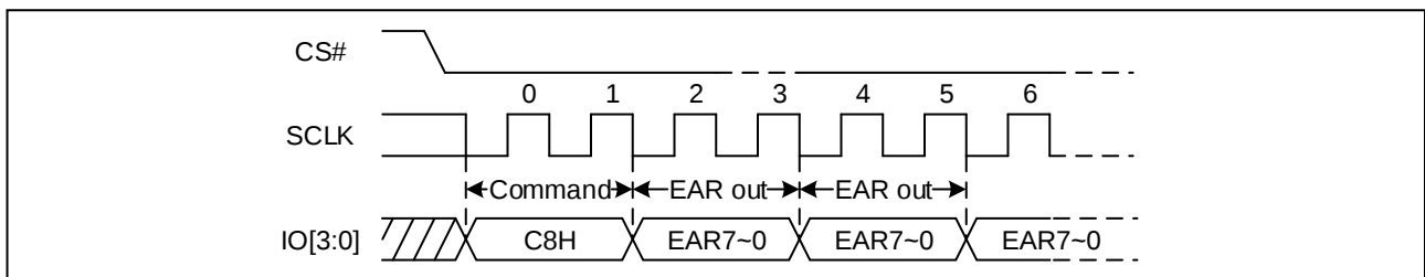
Figure 33 Read Extended Address Register Sequence Diagram (QPI)
