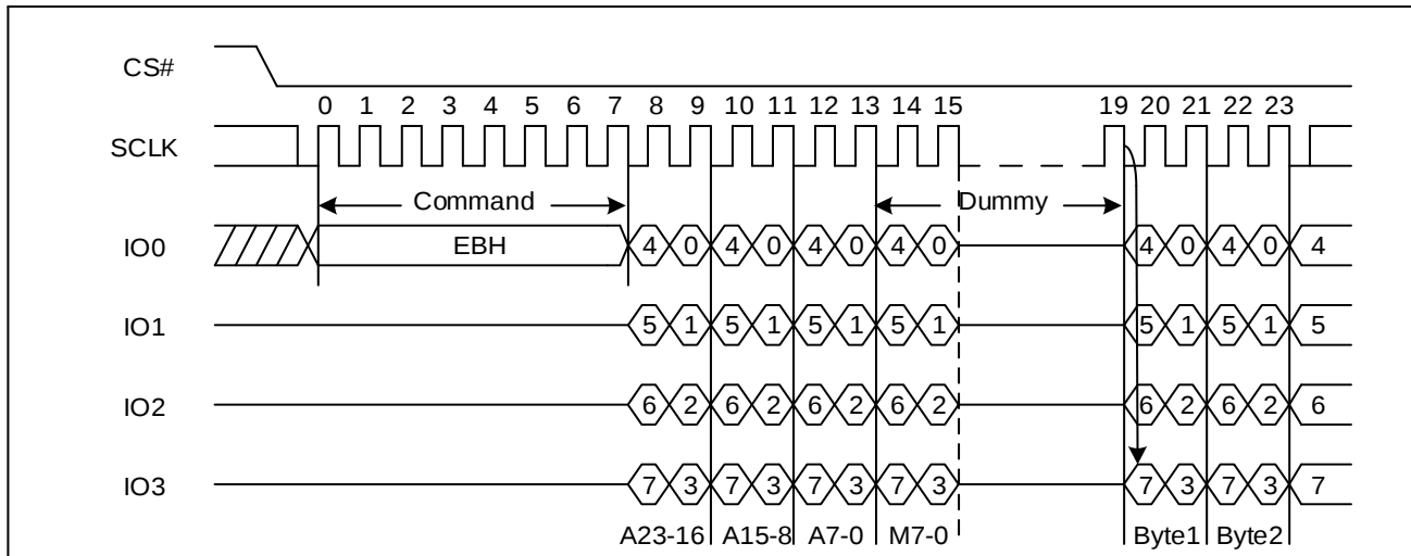
Figure 41 Quad I/O Fast Read Sequence Diagram (SPI, M5-4≠ (1, 0))
