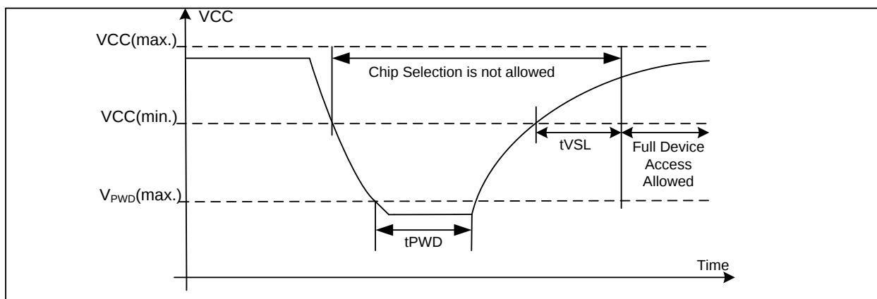
Figure 94. Power-On Timing Sequence Diagram
