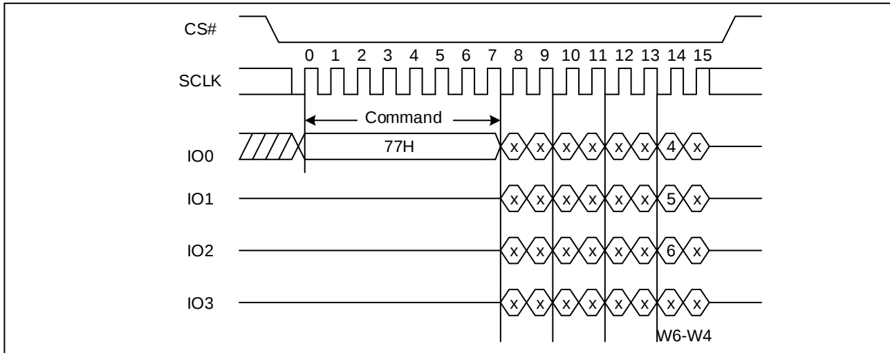
Figure 45. Set Burst with Wrap Sequence Diagram
