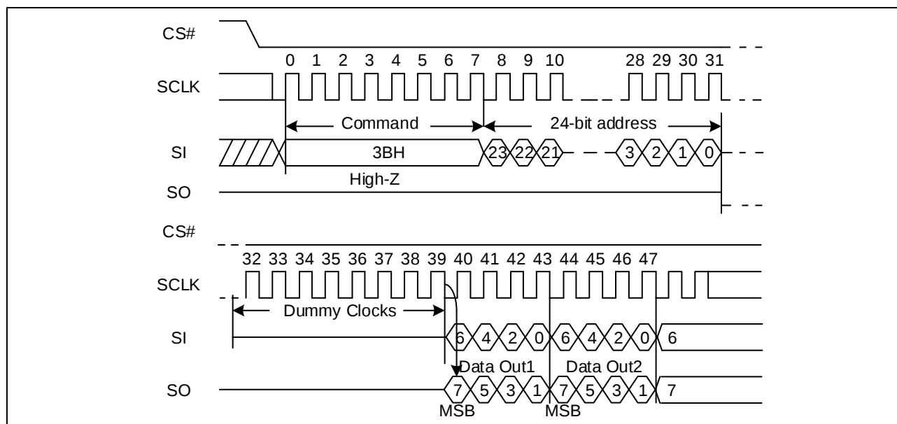
Figure 37. Dual Output Fast Read Sequence Diagram
