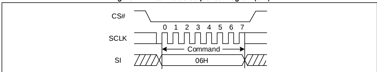
Figure 12 Write Enable Sequence Diagram (SPI)
