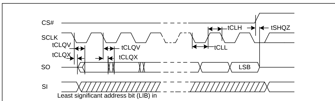
Figure 98. Output Timing
