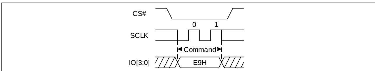
Figure 9 Disable 4-Byte Mode Sequence Diagram (QPI)
