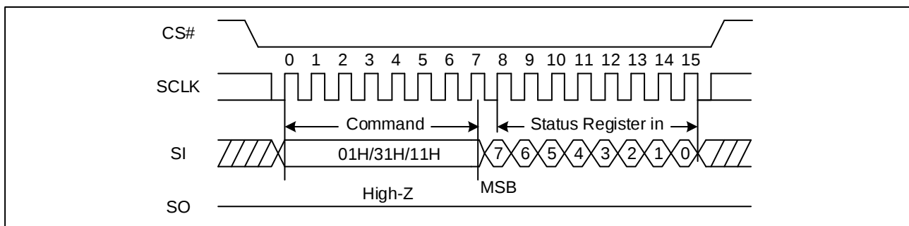
Figure 18 Write Status Register Sequence Diagram (SPI)
