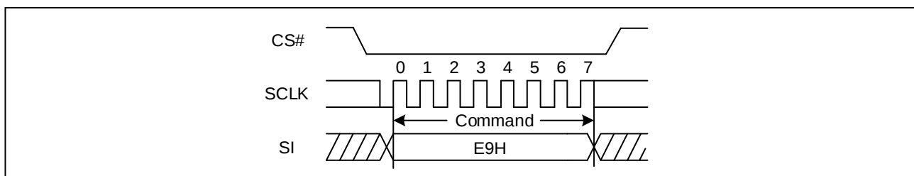
Figure 8 Disable 4-Byte Mode Sequence Diagram (SPI)
