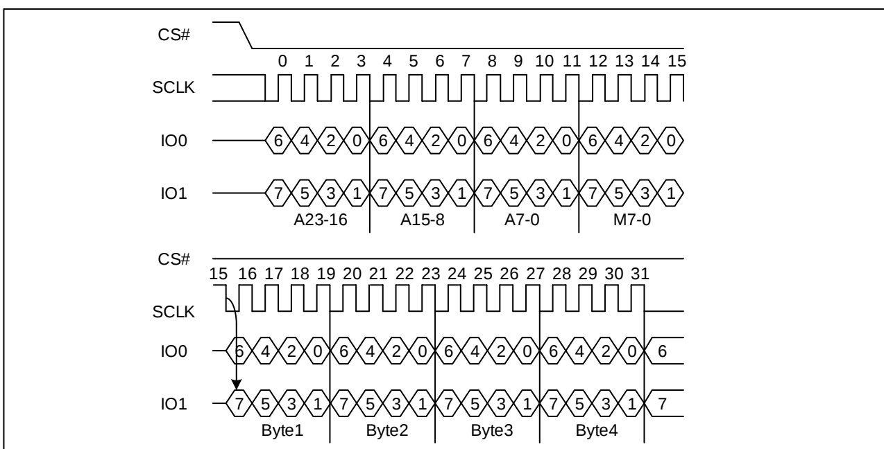
Figure 40 Dual I/O Fast Read Sequence Diagram ((M5-4) = (1, 0))
