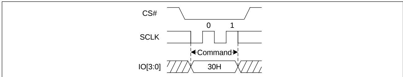
Figure 11. Clear Status Register Flags Diagram (QPI)
