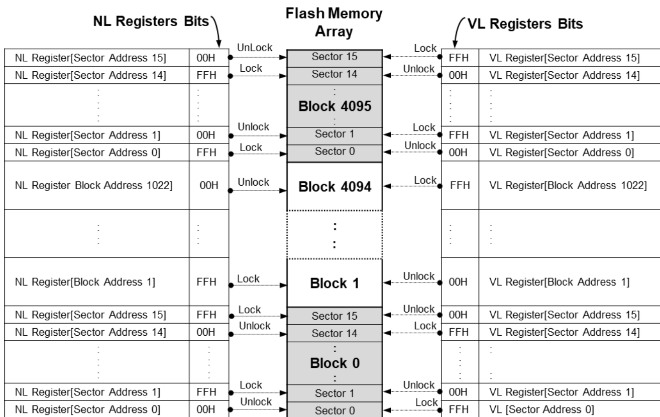
Figure 5. NL Registers and VL Registers Assignment on the Memory
