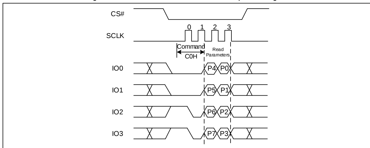
Figure 46. Set Read Parameters command Sequence Diagram
