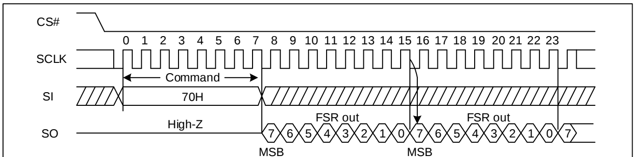
Figure 28 Read Flag Status Register Sequence Diagram (SPI)
