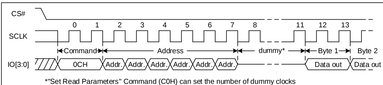
Figure 44. Burst Read with Wrap Sequence Diagram
