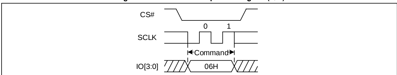
Figure 13 Write Enable Sequence Diagram (QPI)
