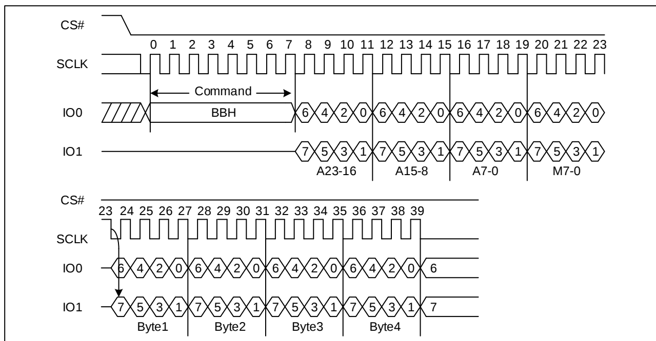
Figure 39 Dual I/O Fast Read Sequence Diagram ((M5-4) ≠ (1, 0))
