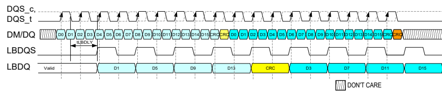
Figure 173 — Loopback Normal Output Mode 4-Way PhaseB with CRC, no Gap Example
