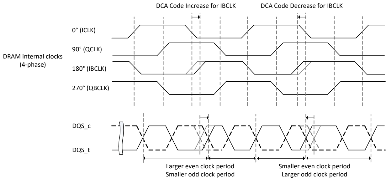
Figure 184 — Relationship between DCA Code Change for IBCLK and the 4-phase internal clocks/DQS waveform (Example)
