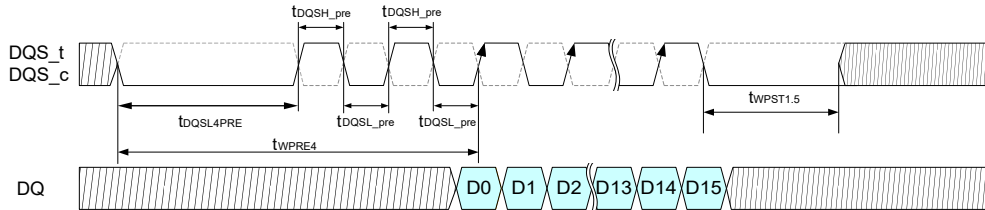
Figure 17 — DQS Timing While 4tCK Write Preamble and 1.5tCK Postamble
