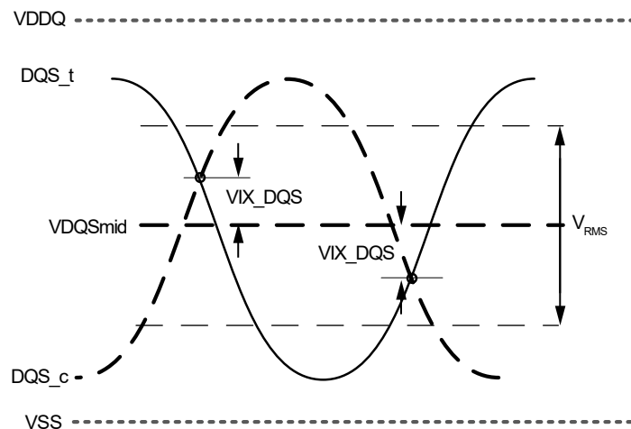
Figure 231 — VIX Definition (DQS)
