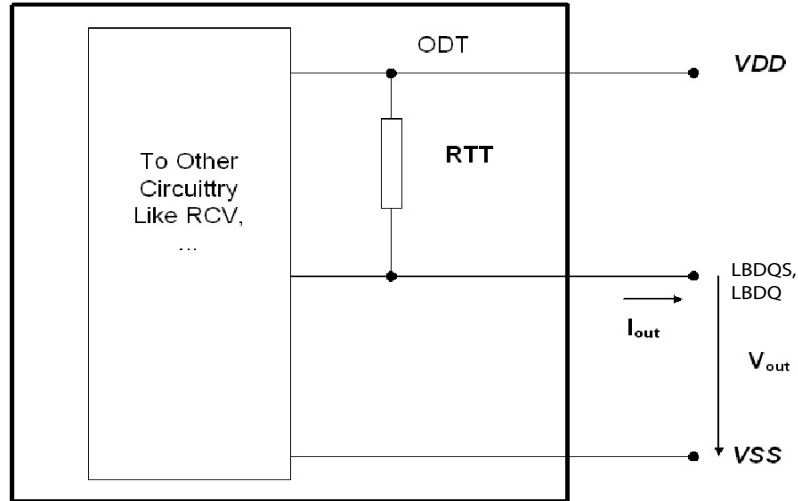
Figure 206 — Functional Representation of Loopback ODT
