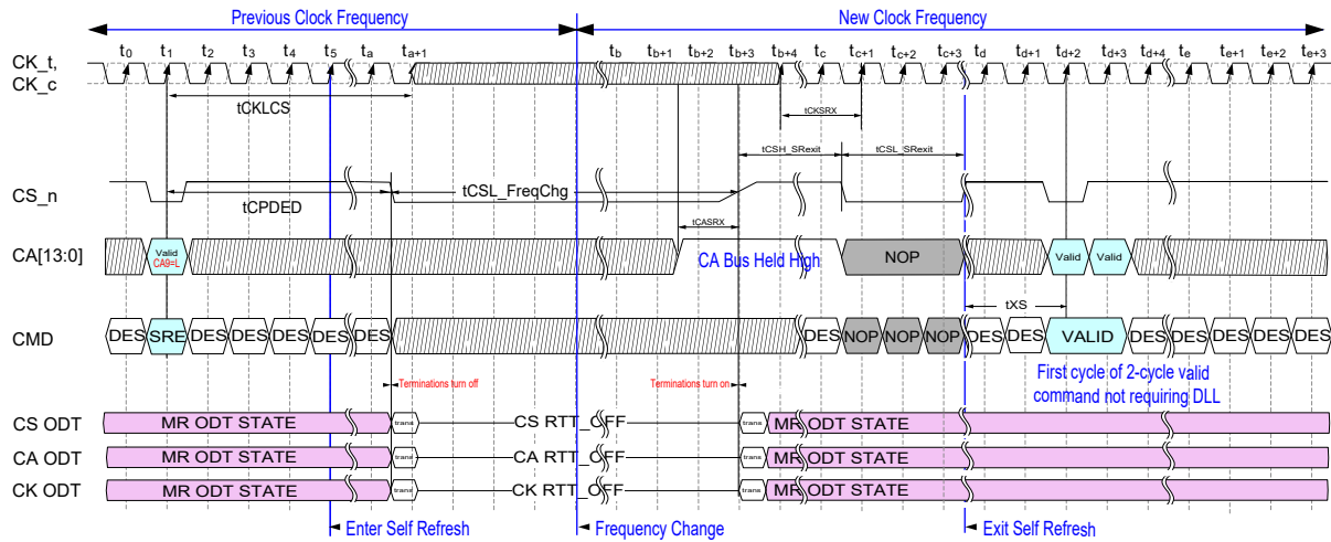
Figure 65 — Frequency Change during Self Refresh
