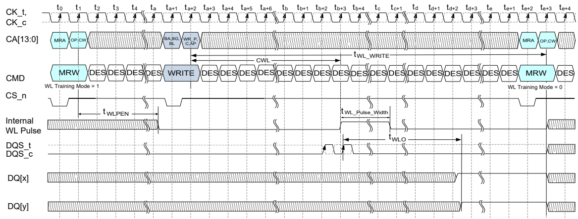
Figure 106 — Write Leveling Training Mode Timing Diagram (External Training, 1N Mode, 1 Sample)
