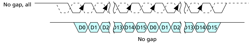
Figure 28 — Example of Seamless Writes Operation: t_{CCD}=\text{Min}
