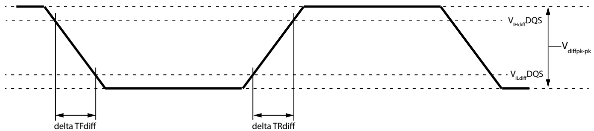
Figure 234 — Differential Input Slew Rate Definition for DQS_t, DQS_c
