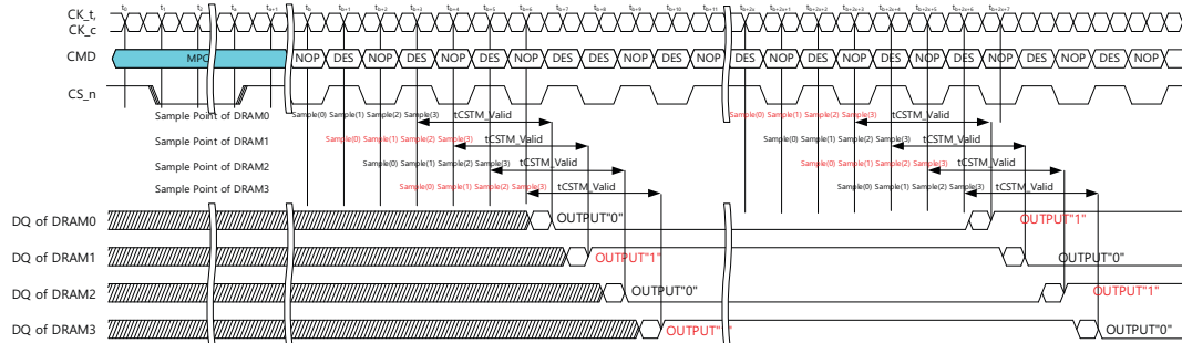
Figure 102 — Timing Diagram for CS Training Mode with Multiple DRAMs Output Sample Toggle
