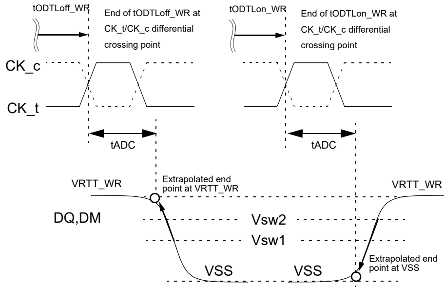
Figure 208 — tADC Measurement Method Target DRAM Write
