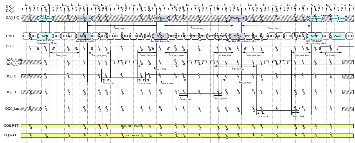
Figure 83 — Multi-Device PDA Enumerate Programming in Legacy Mode with all DQSs
