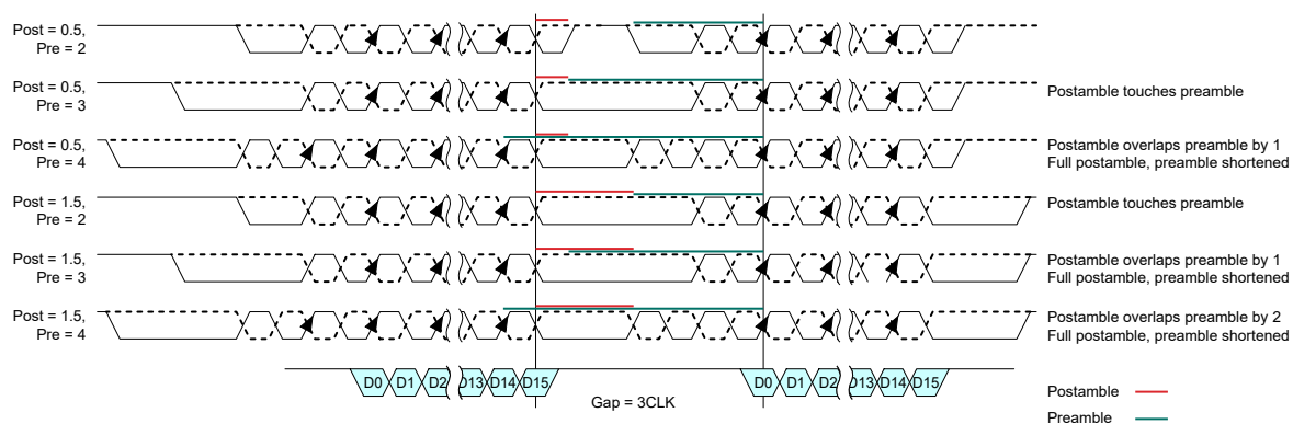
Figure 31 — Example of Consecutive Writes Operation: t_{CCD} = \text{Min} + 3
