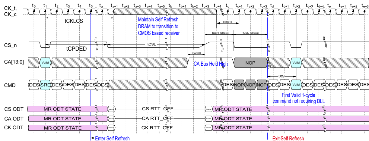
Figure 62 — Self-Refresh Entry/Exit Timing w/ 1-Cycle exit command
