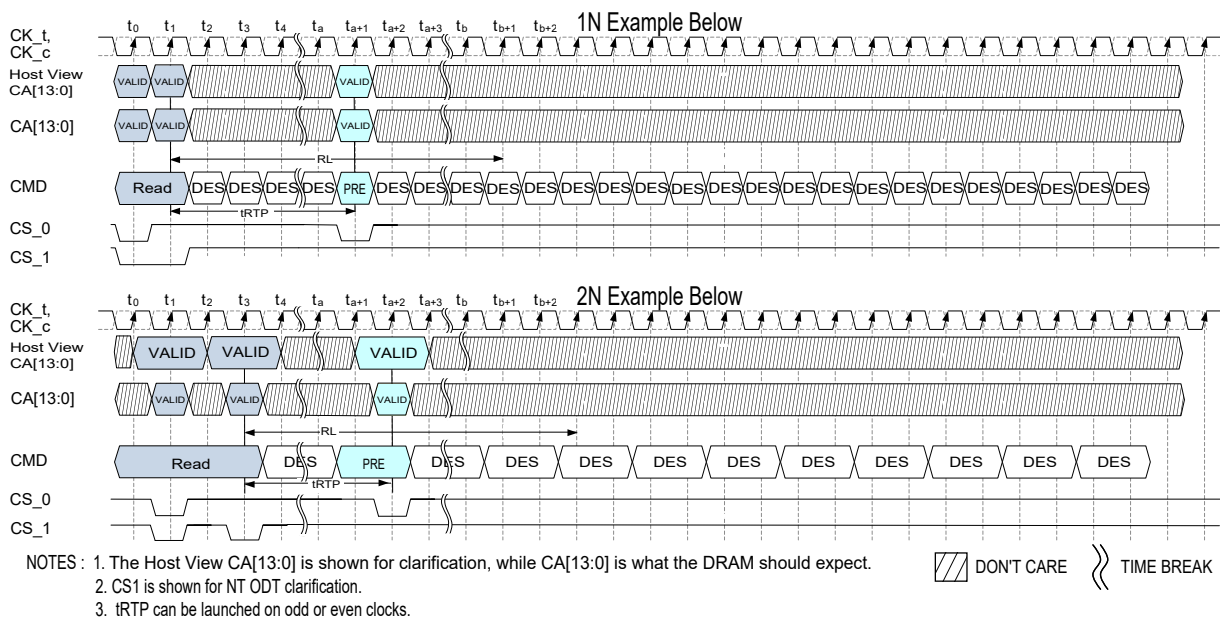
Figure 155 — Example of 1N vs 2N Mode - For reference only
