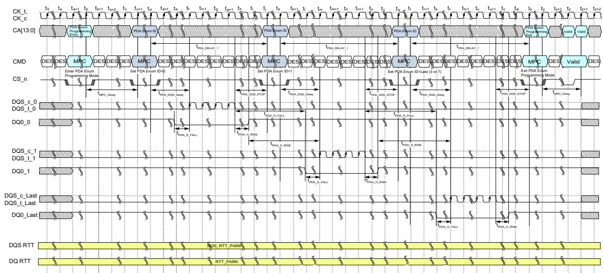
Figure 82 — Multi-Device PDA Enumerate Programming in Legacy Mode with dedicated DQS
