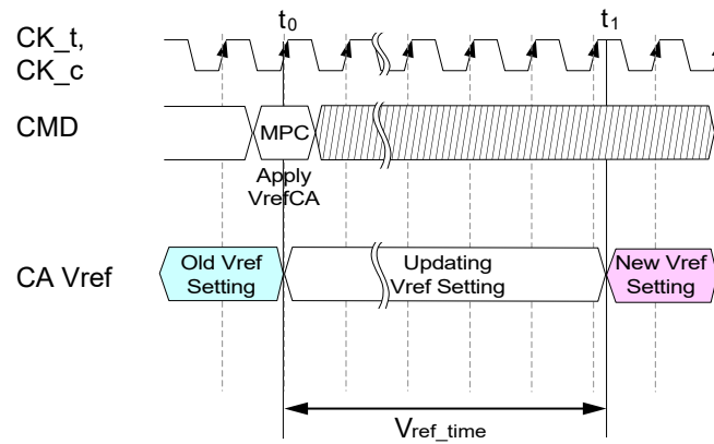
Figure 120 — Vref_time timing diagram
