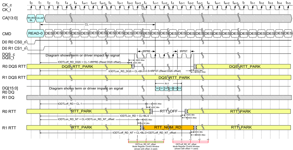
Figure 202 — Example of Burst Read Operation ODT Latencies and Control Diagrams
