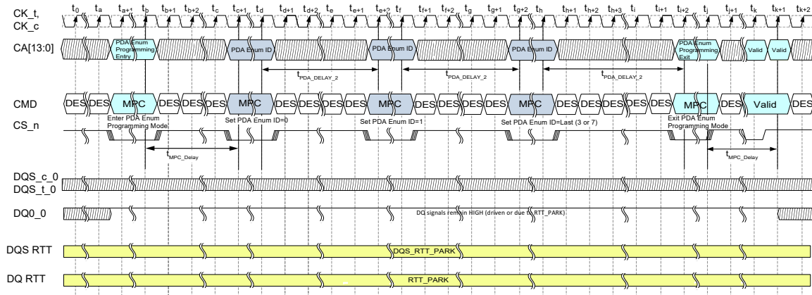
Figure 91 — Multi Device PDA Enumerate Programming “Don’t Enumerate” Case for DQ Held HIGH and any DQS State
