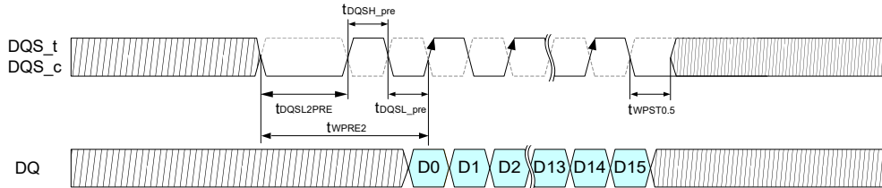
Figure 16 — DQS Timing While 2tCK Write Preamble and 0.5tCK Postamble
