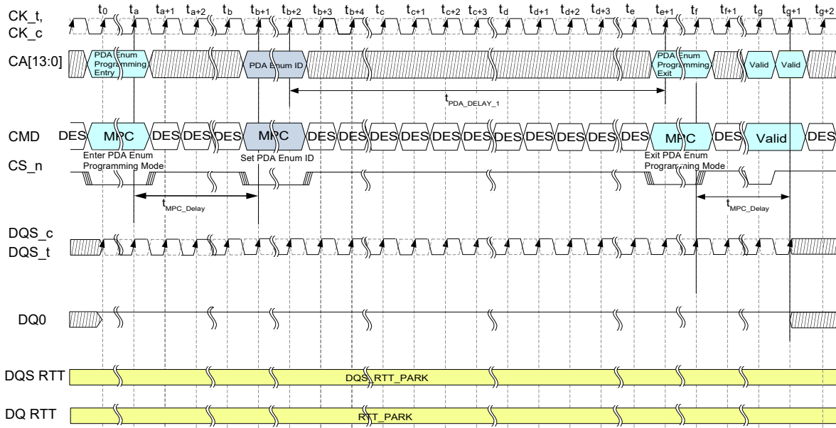
Figure 86 — Single Device PDA Enumerate Programming “Don’t Enumerate” Case in Continuous DQS Toggle Mode
