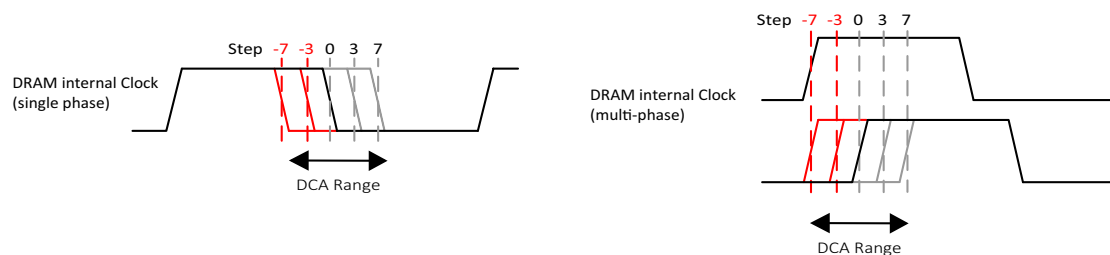
Figure 181 — Duty Cycle Adjuster Range
