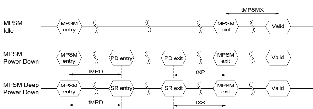
Figure 67 — Maximum Power Saving Mode exit timings
