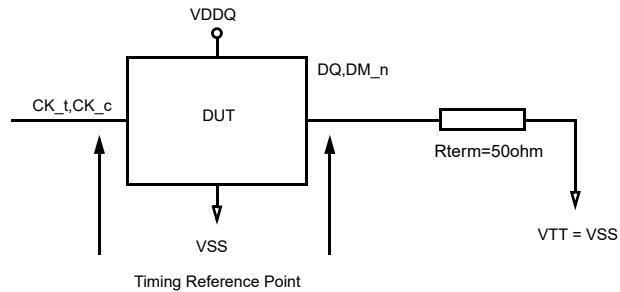
Figure 207 — ODT Timing Reference Load
