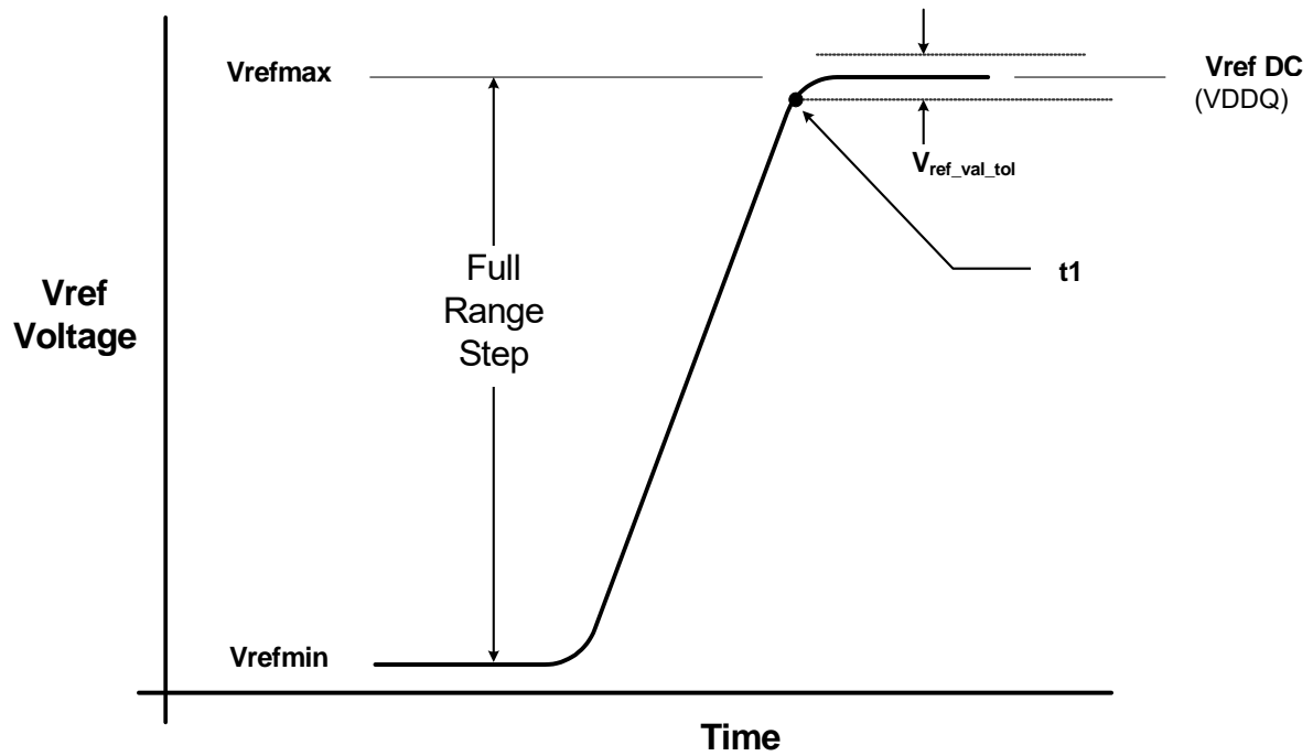
Figure 130 — Vref full step from Vrefmin to Vrefmax case
