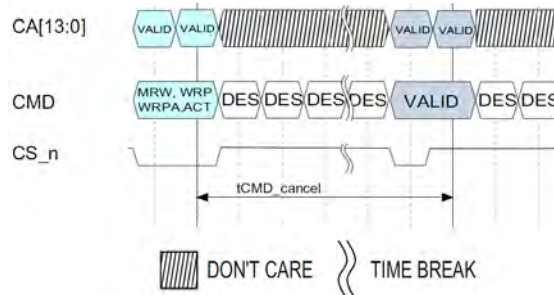
Figure 10 — Command Cancel Timing
