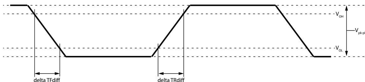
Figure 244 — Single-ended Output Slew Rate Definition
