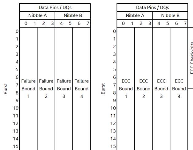
Figure 255 — Example of Fault Boundaries versus on-die ECC data blocks
