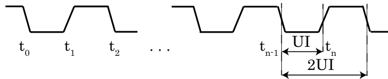
Figure 214 — UI Definition Using Clock Waveforms
