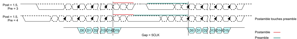
Figure 27 — Example of Consecutive Reads Operation: t_{CCD} = \text{Min} + 5
