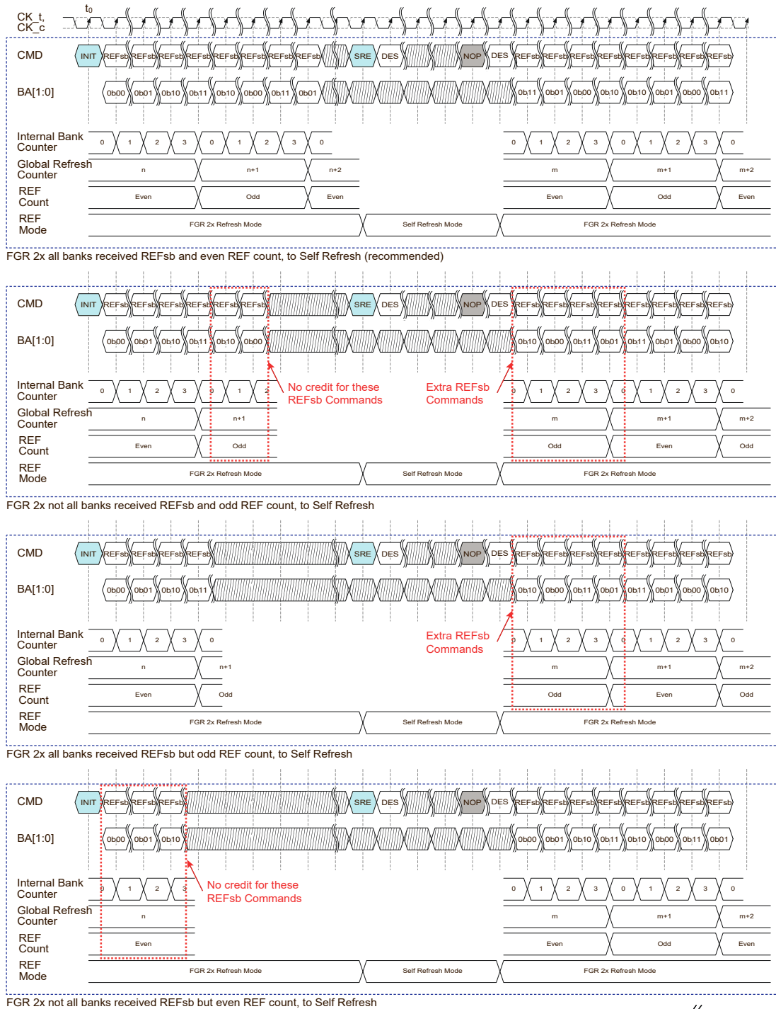
Figure 76 — 16Gb and Higher Density DRAM FGR 2x REFsb to SREF Command Timing
