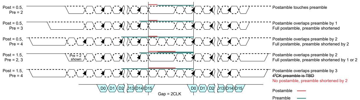
Figure 30 — Example of Consecutive Writes Operation: t_{CCD}=\text{Min}+2
