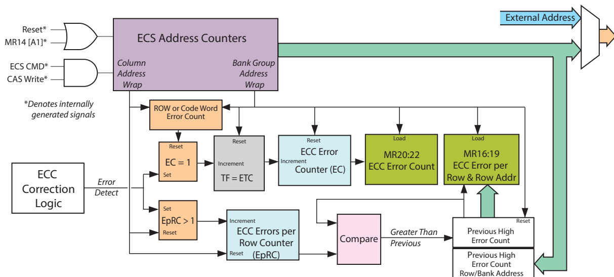
Figure 158 — Example of an ECC Transparency and Error Scrub Functional Block Diagram
