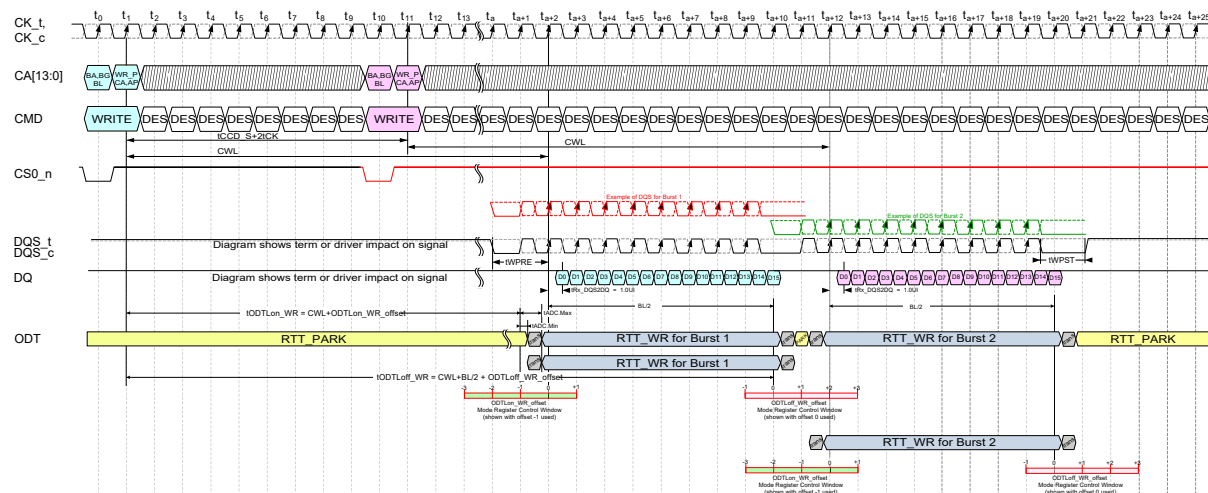
Figure 199 — WRITE (BL16) to WRITE (BL16), Different Bank, 2 tCK Gap
