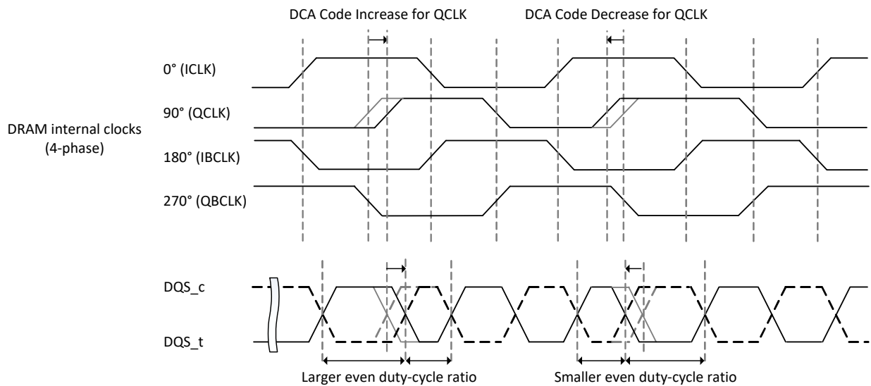
Figure 183 — Relationship between DCA Code Change for QCLK and the 4-phase internal clocks/DQS waveform (Example)
