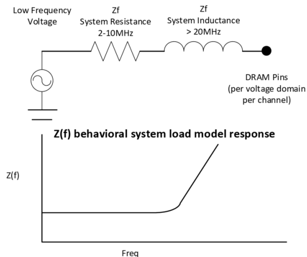
Figure 212 — Simplified Z(f) electrical model and frequency response of PDN at the DRAM pin without the DRAM component
