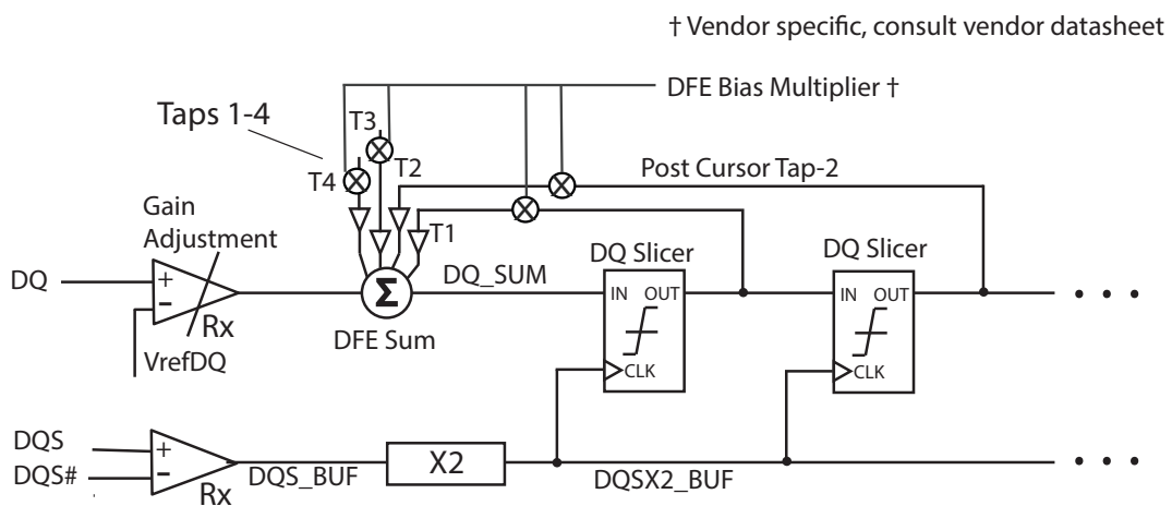
Figure 147 — 4-Tap DFE Example
