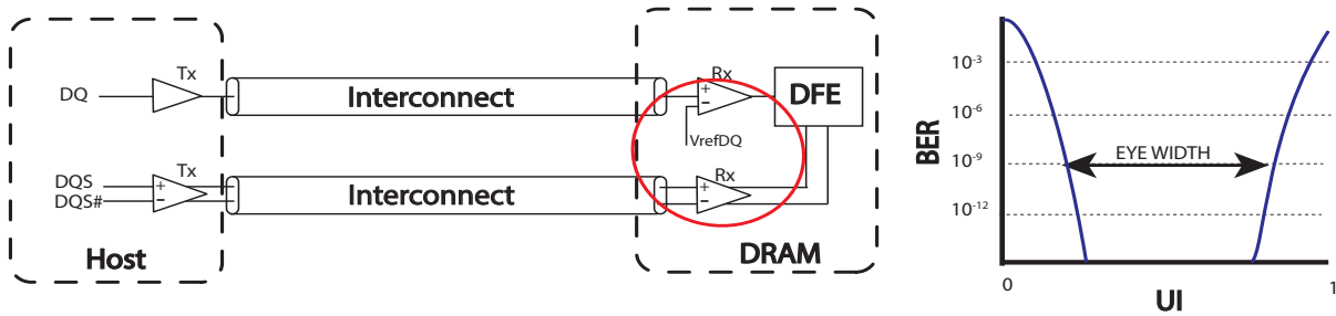
Figure 228 — SDRAM's Rx Forwarded Strokes for Jitter Sensitivity Testing
