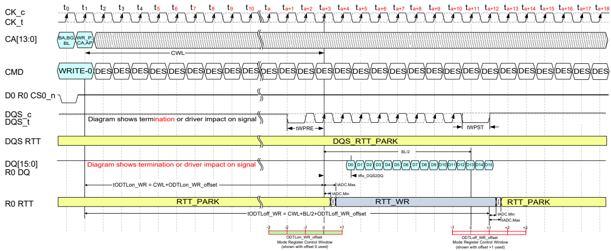
Figure 194 — Example 3 of Burst Write Operation ODT Latencies and Control Diagrams
