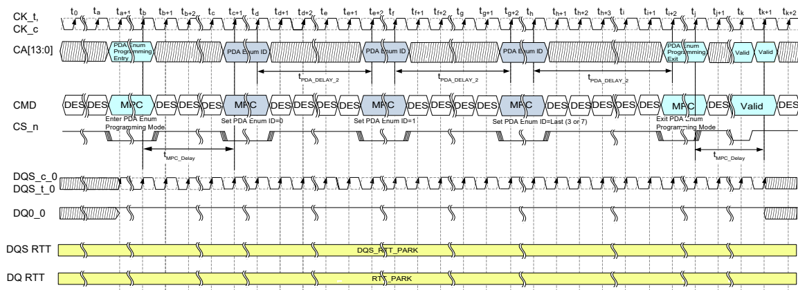
Figure 90 — Multi Device PDA Enumerate Programming “Don’t Enumerate” Case in Continuous DQS Toggle Mode
