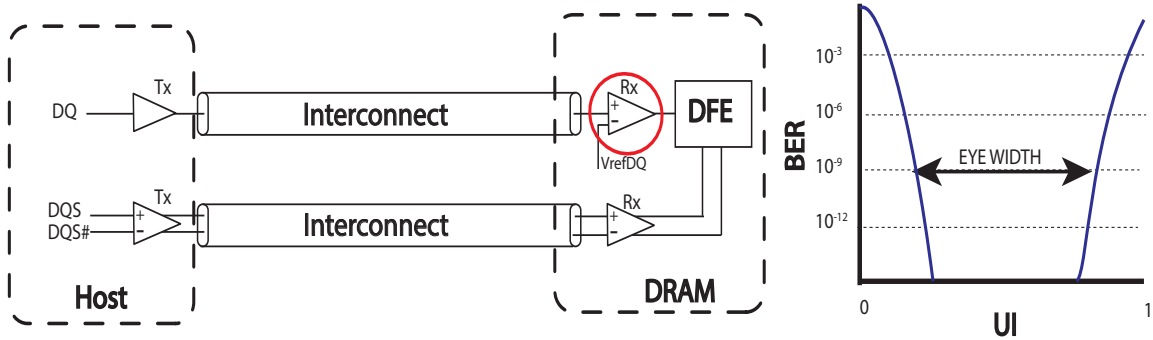
Figure 232 — Example of DDR5 Memory Interconnect
