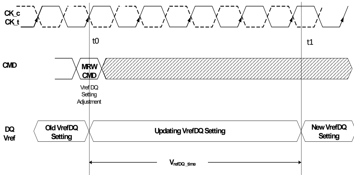
Figure 134 — VrefDQ_time timing diagram
