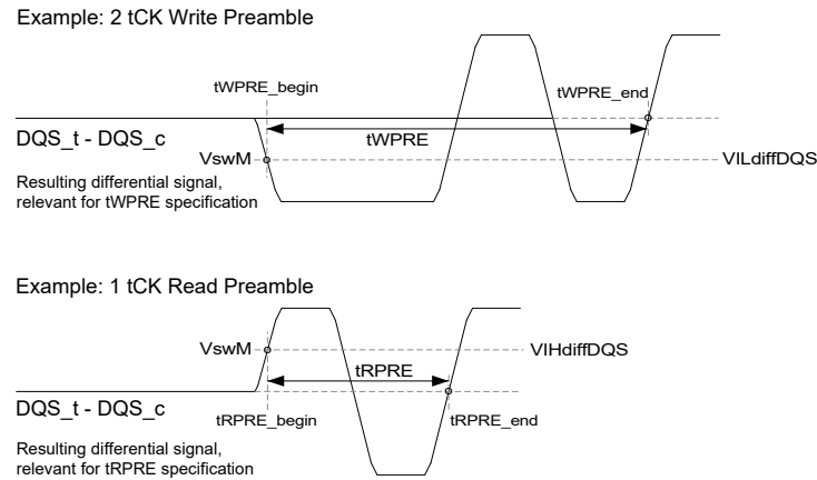
Figure 20 — Method for measuring Preamble start and end points
