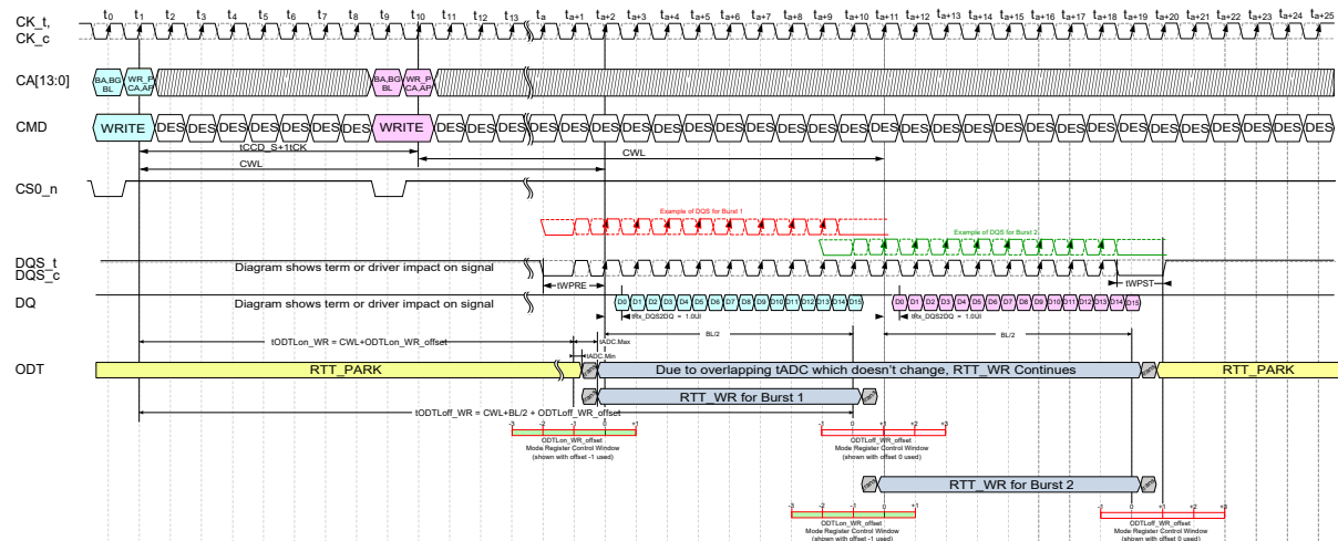
Figure 198 — WRITE (BL16) to WRITE (BL16), Different Bank, 1 tCK Gap
