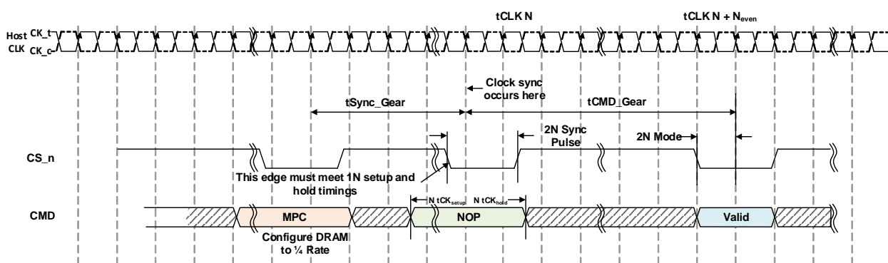
Figure 186 — Geardown during Initializations
