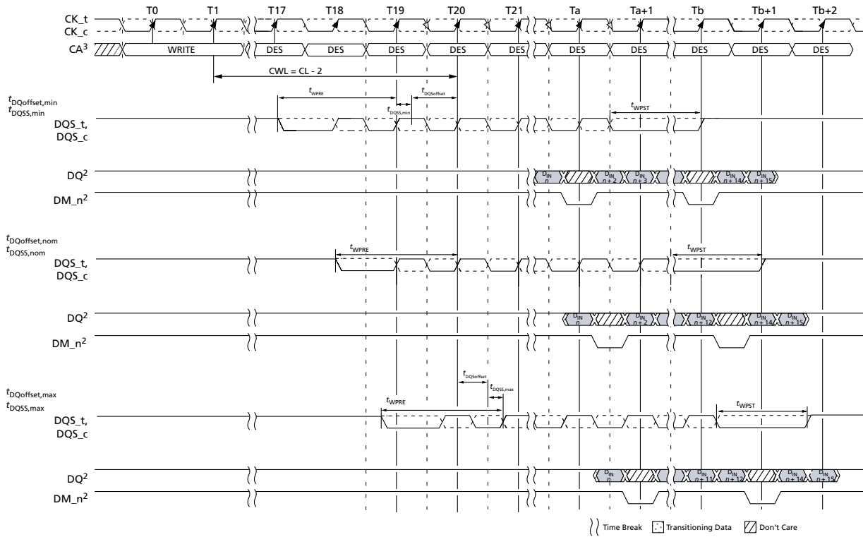
Figure 52 — DDR5 Write Timing Parameters
