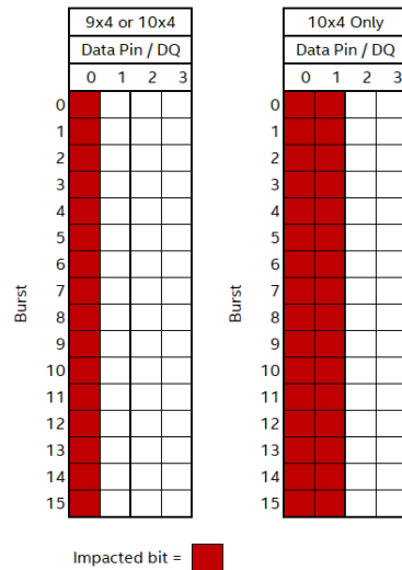
Figure 254 — Example of x4 Fault Boundary.
