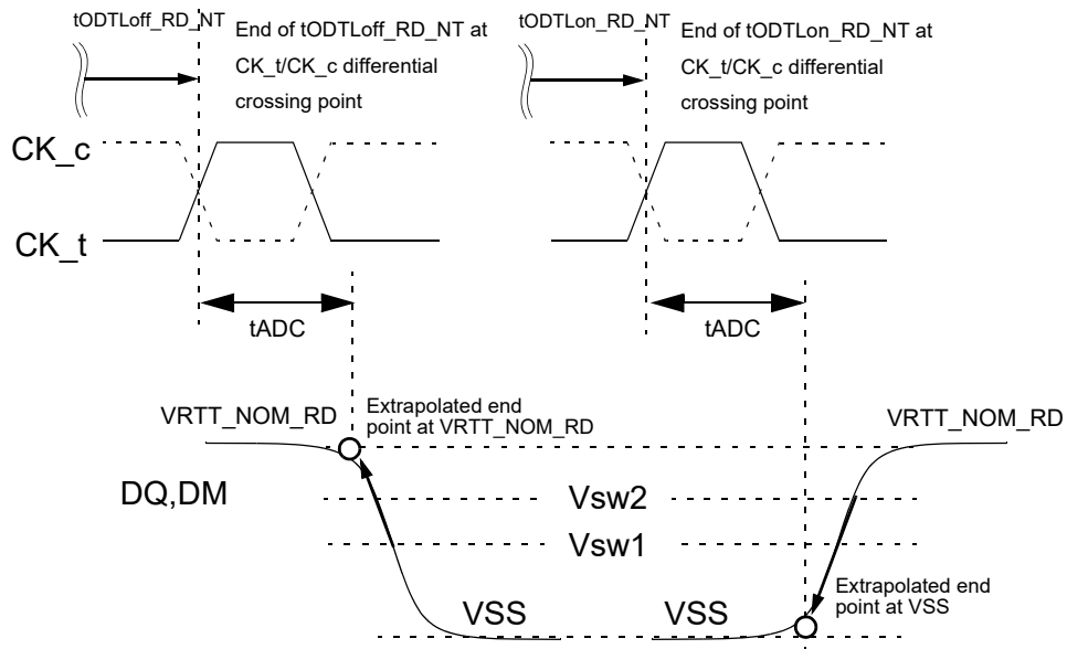
Figure 210 — t_{ADC} Measurement Method Non-Target DRAM Read
