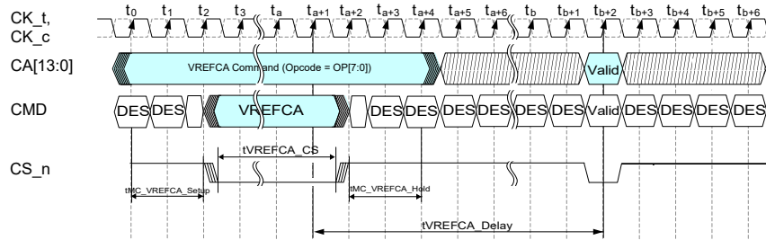
Figure 116 — Timing Diagram for VrefCA Command
