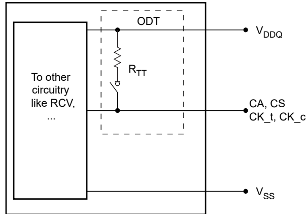
Figure 204 — A simple functional representation of the DRAM CA ODT feature
