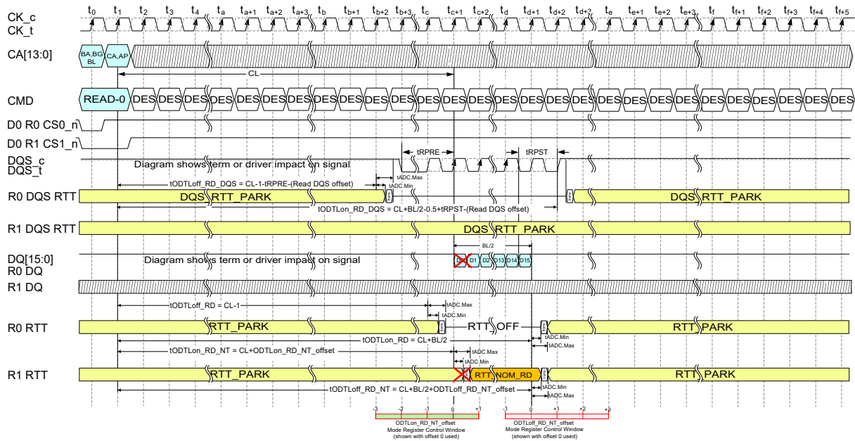
Figure 203 — Example of Burst Read Operation with ODTLon_RD_NT_offset set incorrectly
