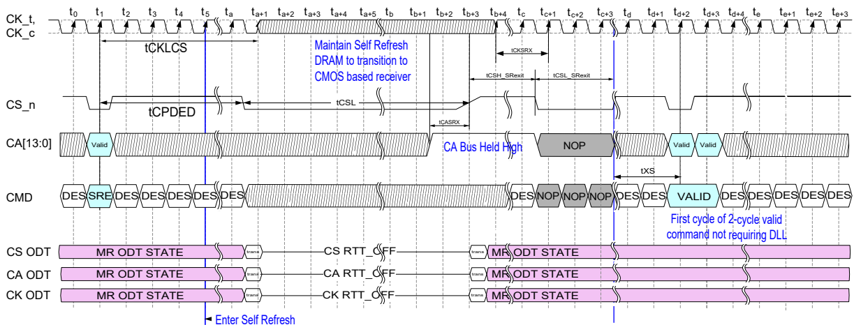
Figure 61 — Self-Refresh Entry/Exit Timing w/ 2-Cycle exit command
