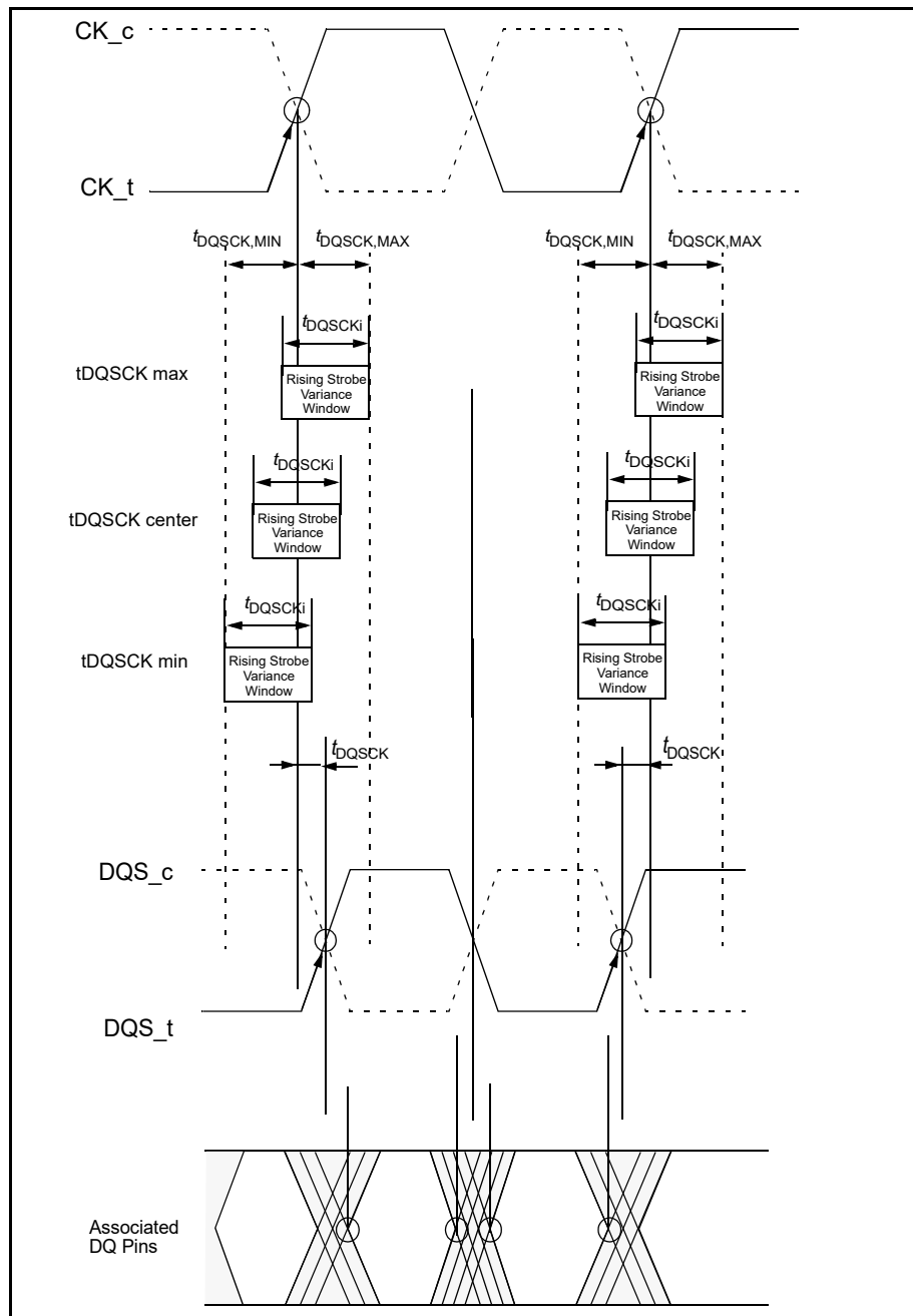
Figure 39 — TDQSCK Timing Definition
