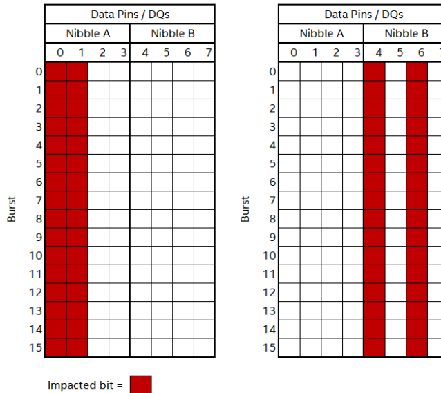
Figure 253 — Examples of x8 Fault Boundaries
