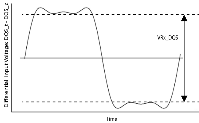
Figure 230 — VRx_DQS
