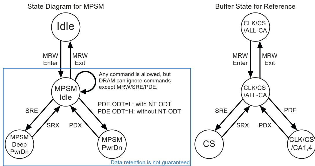
Figure 66 — State diagram for Maximum Power Saving Mode
