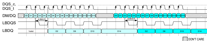
Figure 172 — Loopback Normal Output Mode 4-Way PhaseC 2CK Gap Example
