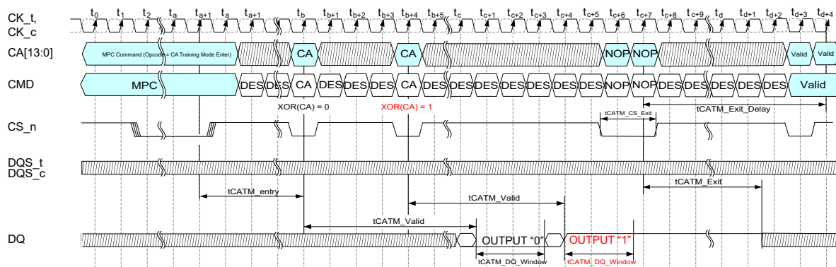
Figure 99 — Timing Diagram for CA Training Mode
