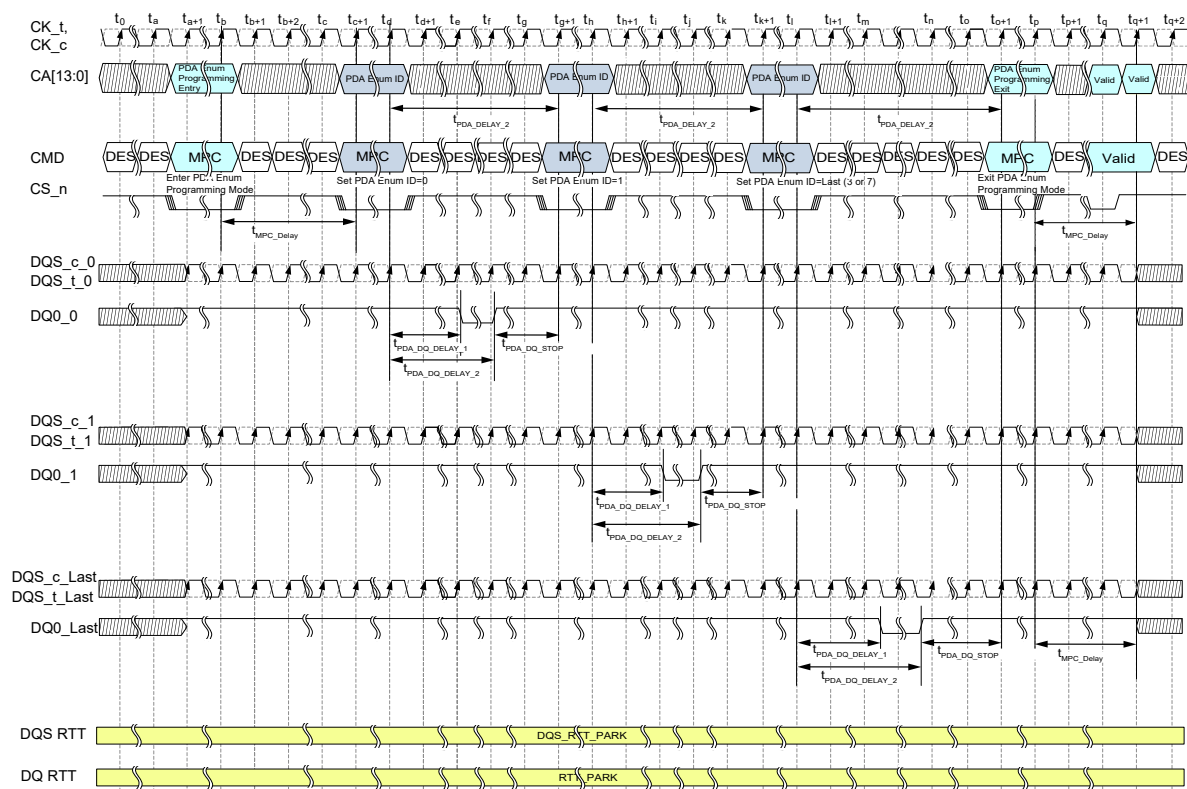
Figure 84 — Multi-Device PDA Enumerate Programming in Continuous DQS Toggle Mode
