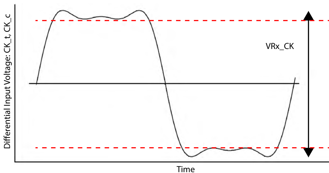
Figure 226 — VRx_CK
