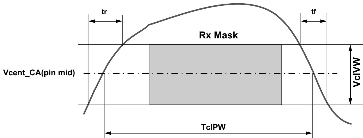
Figure 222 — CA TcIPW and SRIN_cIVW definition (for each input pulse)
