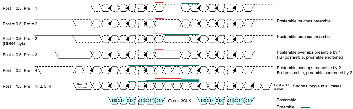
Figure 24 — Example of Consecutive Reads Operation: tCCD=Min+2
