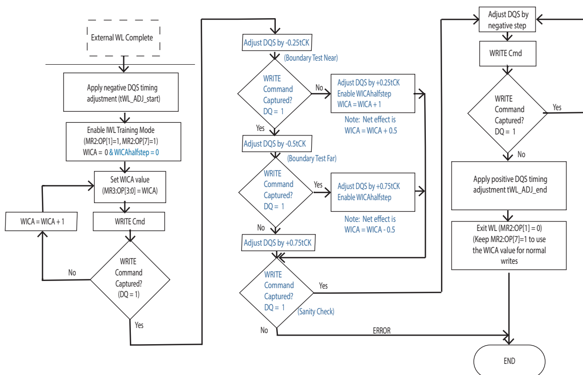
Figure 108 — Write Leveling Training Flow with half step WICA
