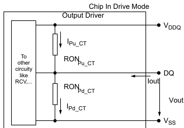
Figure 242 — Output Driver
