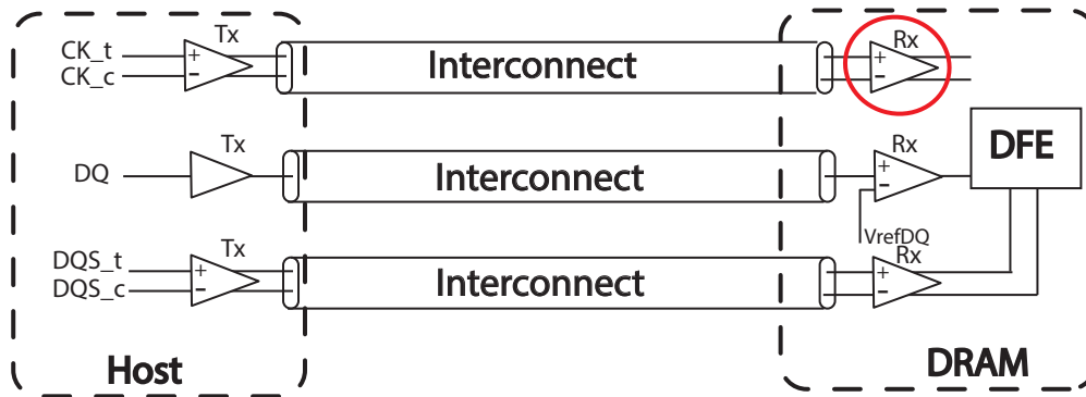
Figure 225 — Example of DDR5 Memory Interconnect
