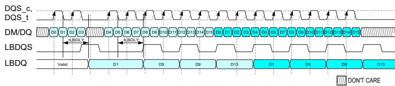
Figure 170 — Loopback Normal Output Mode 4-Way PhaseB 1CK mid Gap Example
