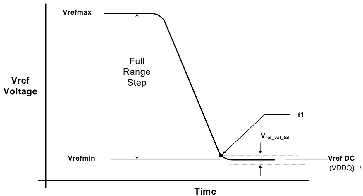
Figure 138 — VrefDQ full step from VrefDQmax to VrefDQmin case.
