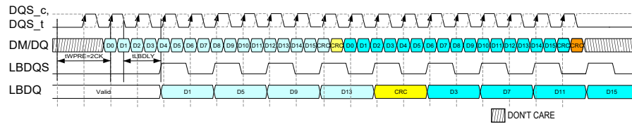
Figure 180 — Loopback Write Burst with CRC Output Mode 4-Way PhaseB with CRC, No Gap Example
