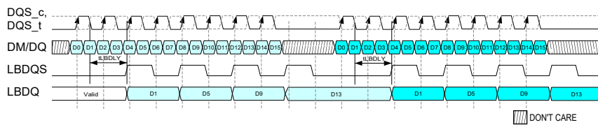
Figure 171 — Loopback Normal Output Mode 4-Way PhaseB 2CK Gap Example
