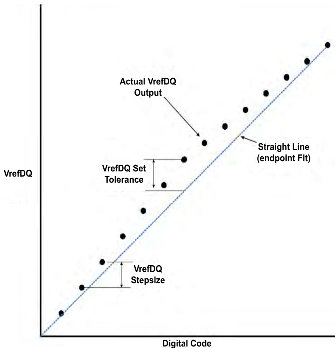
Figure 133 — Example of Vref set tolerance (max case only shown) and stepsize
