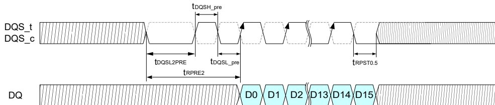
Figure 18 — DQS Timing While 2tCK Read Preamble and 0.5tCK Postamble
