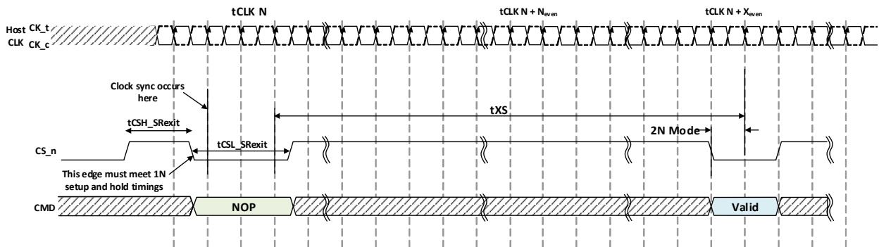
Figure 187 — Geardown Enabled during SRX
