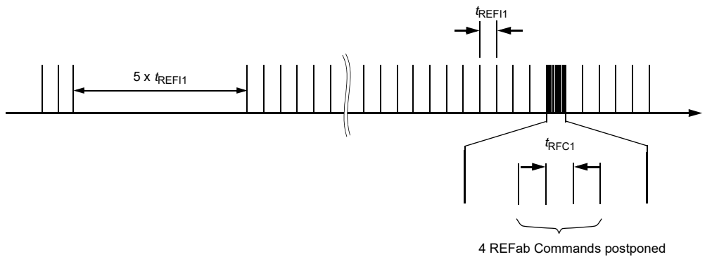
Figure 73 — Postponing Refresh Commands (Example of Normal Refresh Mode - t_{REFI1} , t_{RFC1} )
