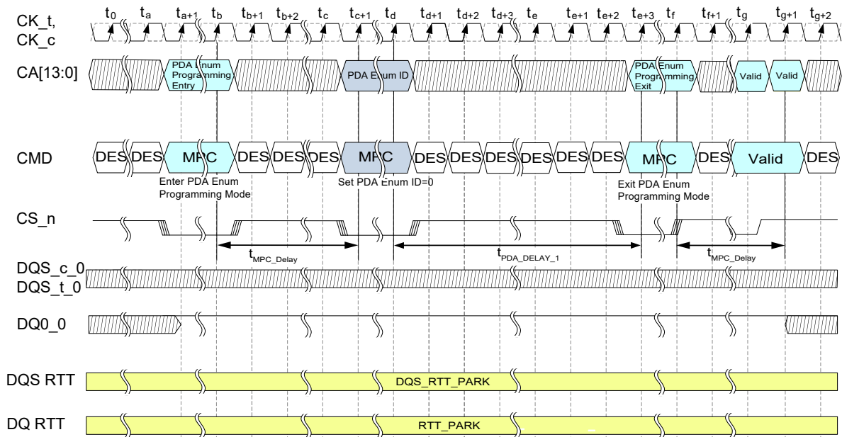
Figure 87 — Single Device PDA Enumerate Programming “Don’t Enumerate” Case for DQ Held HIGH with any DQS State
