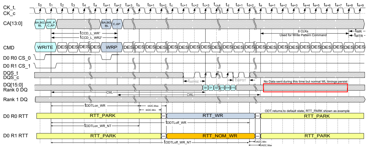
Figure 156 — Example of Write Pattern Command
