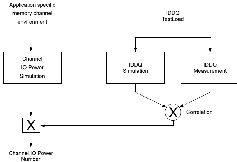
Figure 251 — Correlation from simulated Channel IO Power to actual Channel IO Power supported by IDDQ Measurement.
