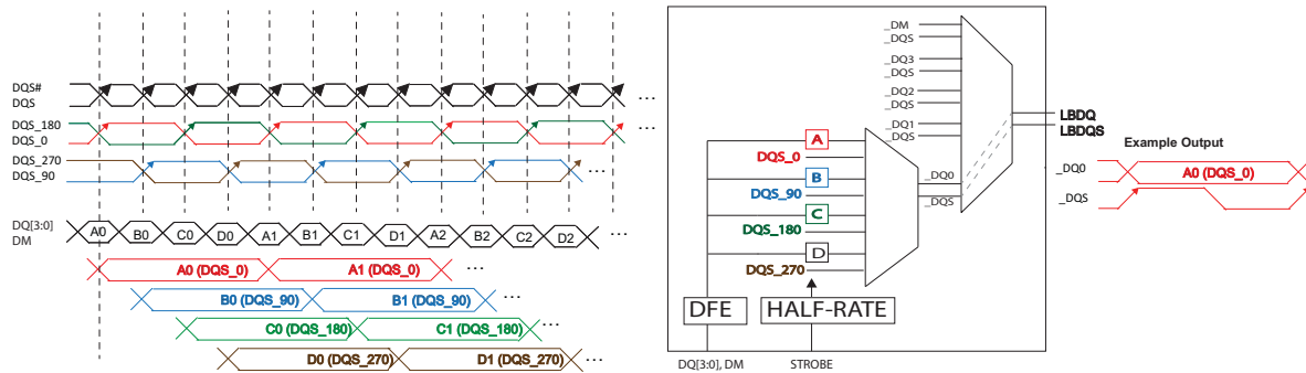
Figure 167 — Example of 4-Way Interleave Loopback Circuit on a x4 SDRAM
