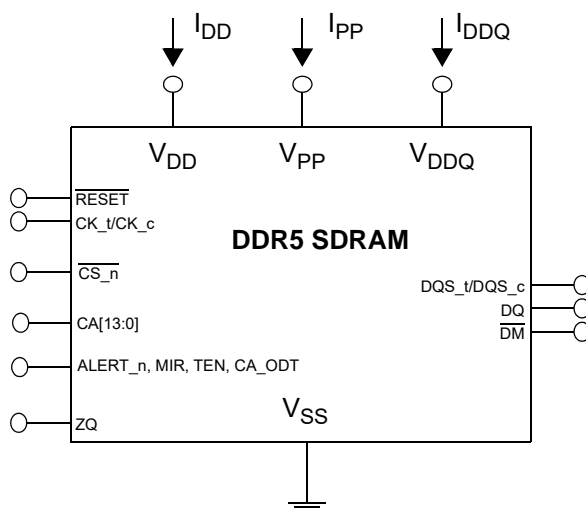
Figure 250 — Measurement Setup and Test Load for IDD, IPP and IDDQ Measurements
