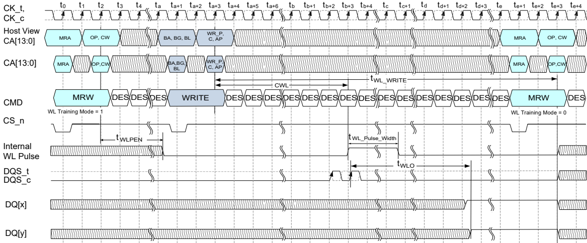
Figure 105 — Write Leveling Training Mode Timing Diagram (External Training, 2N Mode, 1 Sample)
