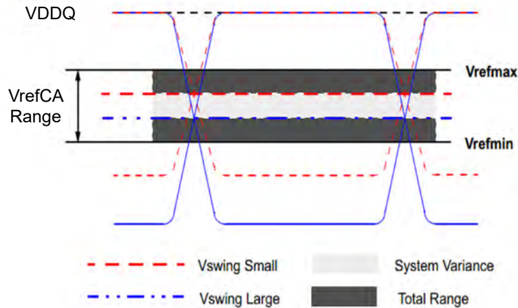
Figure 118 — VrefCA operating range(Vrefmin, Vrefmax)
