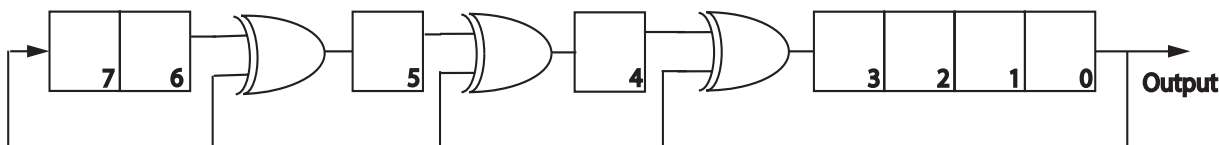
Figure 94 — Read Training Pattern LFSR
