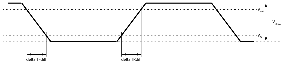
Figure 243 — Single-ended Output Slew Rate Definition
