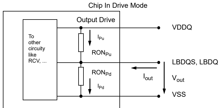
Figure 240 — Output Driver for Loopback Signals
