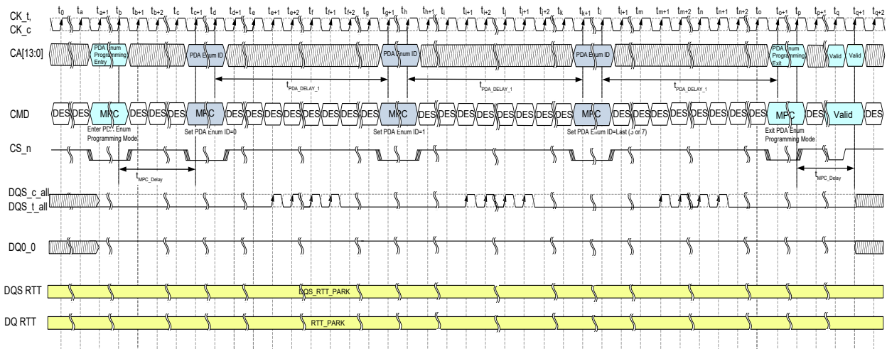
Figure 89 — Multi Device PDA Enumerate Programming “Don’t Enumerate” Case in Legacy Mode
