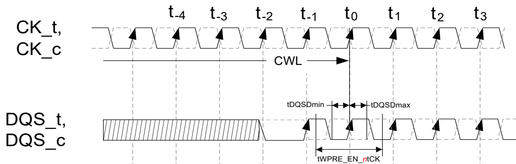
Figure 60 — tDQSD : DRAM internal CLK-to-DQS Variation
