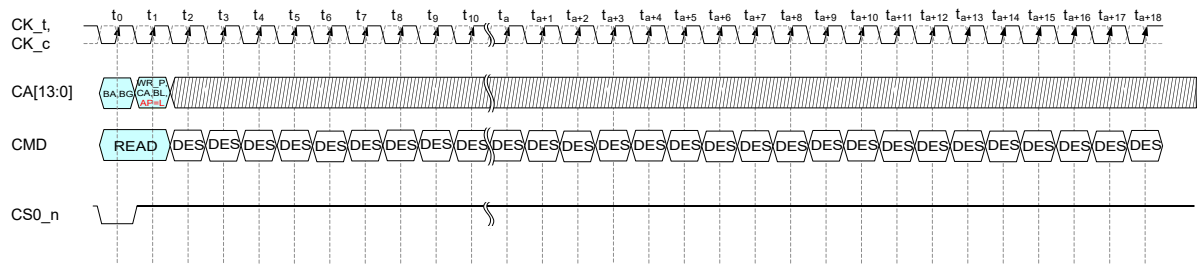
Figure 44 — Read with Auto-Precharge for Fixed BL32 and BL32 in BL32 OTF Mode
