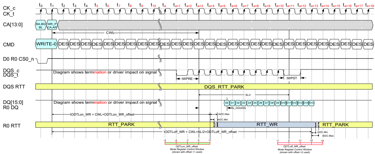
Figure 195 — Example 4 of Burst Write Operation ODT Latencies and Control Diagrams
