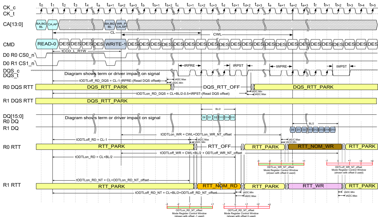
Figure 201 — Example of Read to Write turn around, Different Ranks
