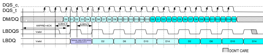
Figure 178 — Loopback Write Burst Output Mode 4-Way PhaseB Data Burst Bit and PhaseD Strobe Alignment WPRE=4CK Optional Example
