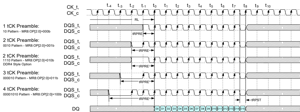
Figure 11 — Example of Read Preamble Modes (default) w/0.5 tCK Postamble
