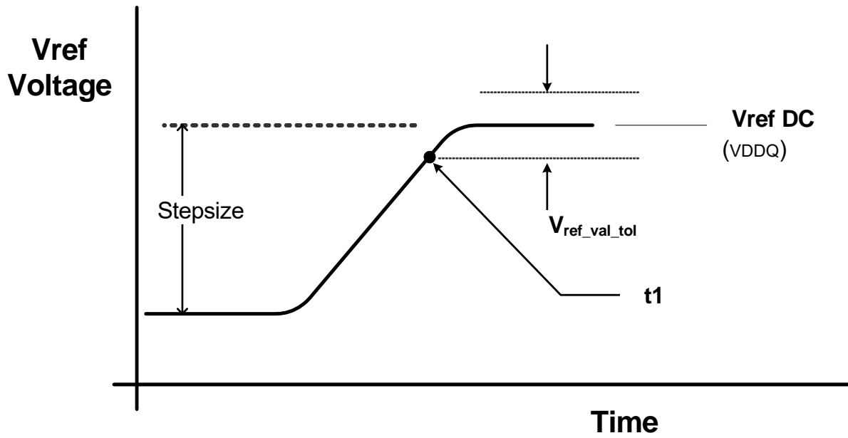
Figure 128 — Vref step single stepsize increment case.
