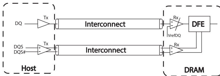
Figure 145 — Example of Memory Subsystem with DFE Circuit on the DRAM
