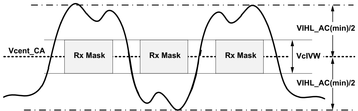
Figure 223 — CA VIH_L_AC definition (for each input pulse)
