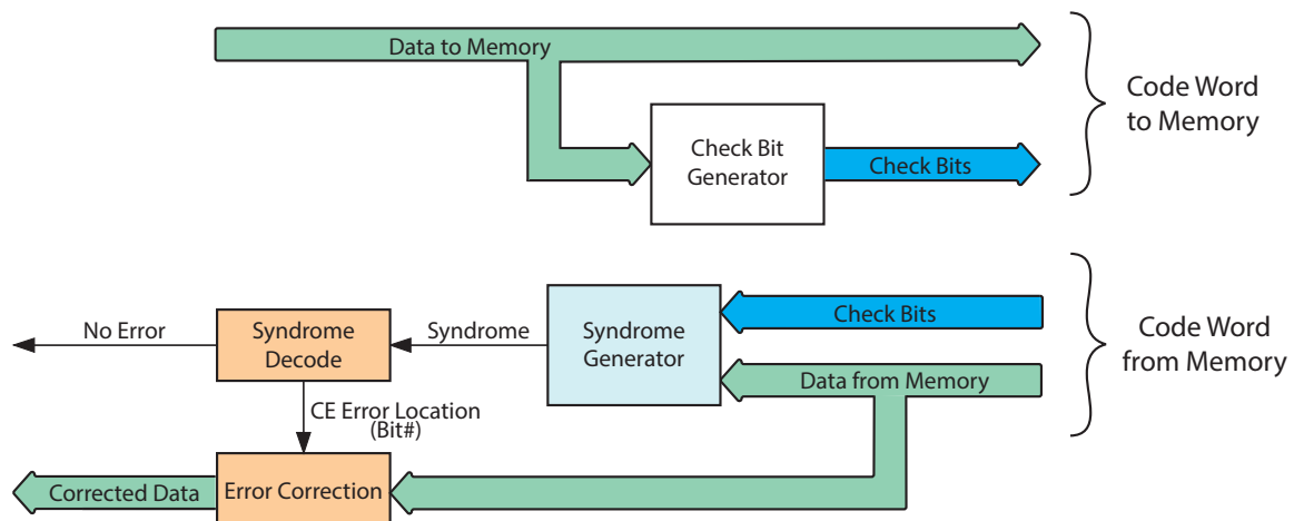
Figure 157 — On Die ECC Block Diagram
