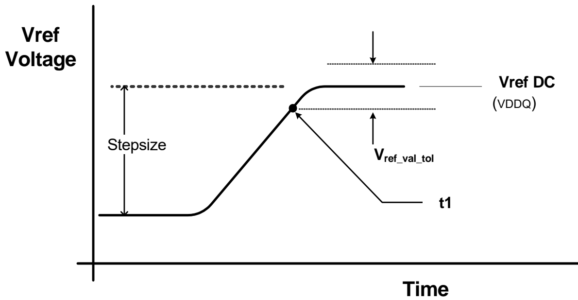
Figure 121 — Vref step single stepsize increment case.
