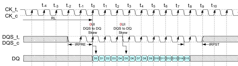
Figure 248 — Read burst example for pin DQx depicting bit 0 and 5 relative to the DQS edge for 0 UI skew
