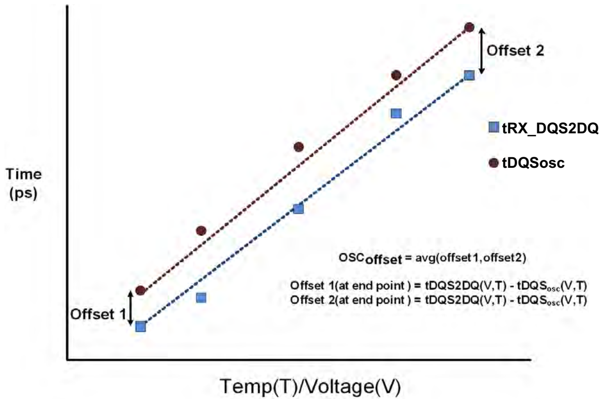
Figure 152 — Interval oscillator offset ( OSC_{Offset} )
