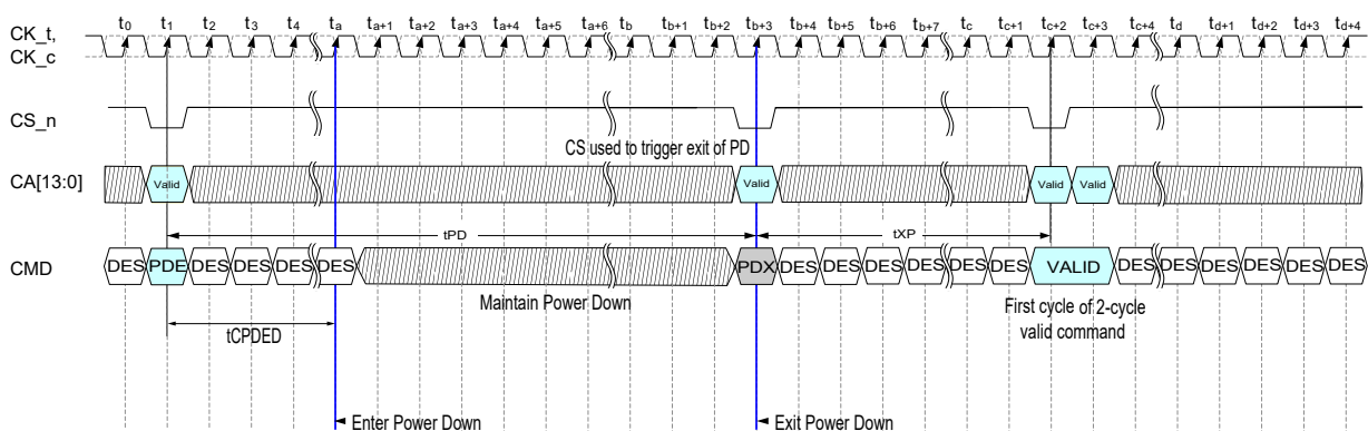
Figure 64 — Power-Down Entry and Exit Mode
