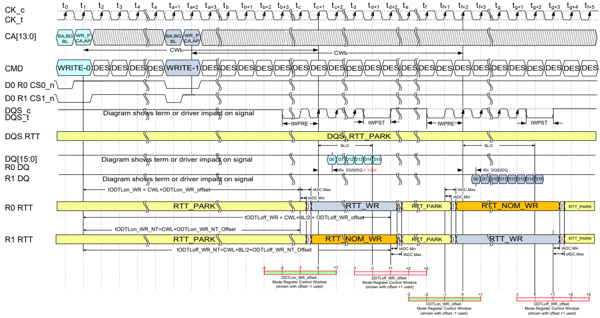
Figure 196 — Example of Write to Write turn around, Different Ranks
