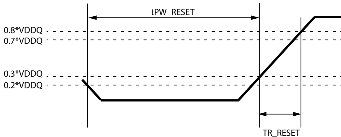
Figure 239 — RESET n Input Slew Rate Definition
