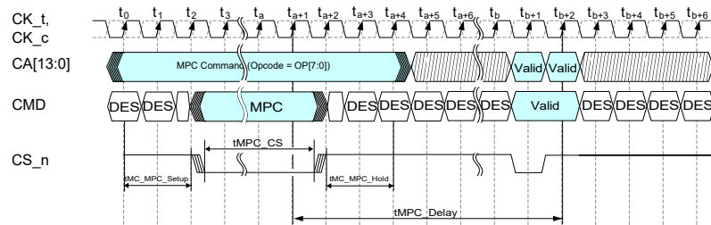
Figure 79 — MPC Function Timing to 2-Cycle Command
