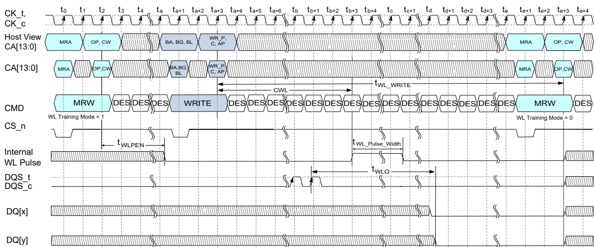
Figure 103 — Write Leveling Training Mode Timing Diagram (External Training, 2N Mode, 0 Sample)
