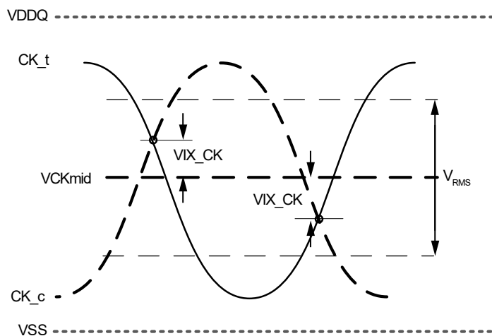
Figure 139 - VIX Definition (CK)
