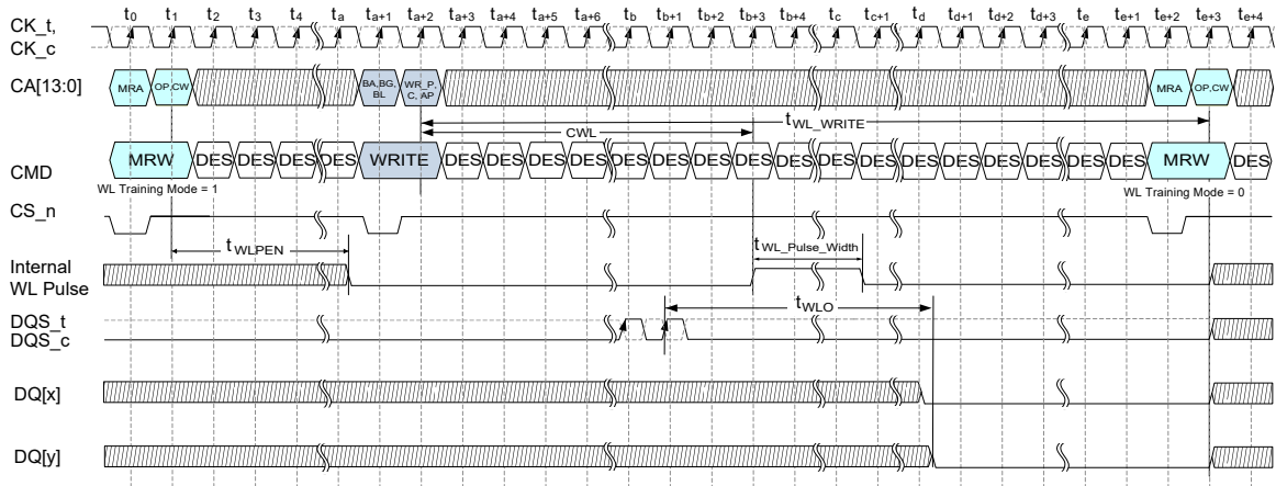
Figure 104 — Write Leveling Training Mode Timing Diagram (External Training, 1N Mode, 0 Sample)
