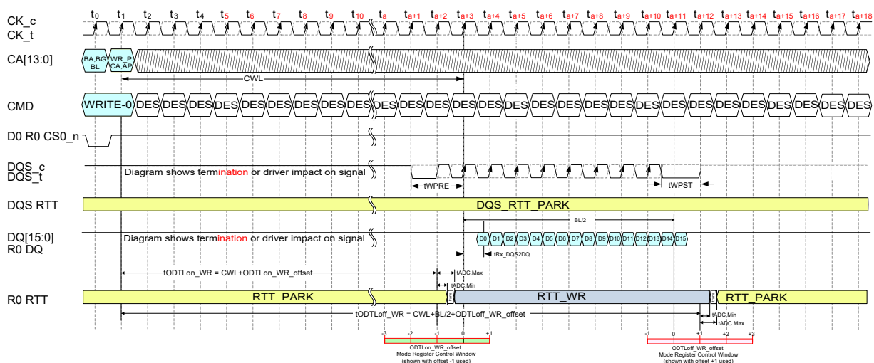
Figure 193 — Example 2 of Burst Write Operation ODT Latencies and Control Diagrams
