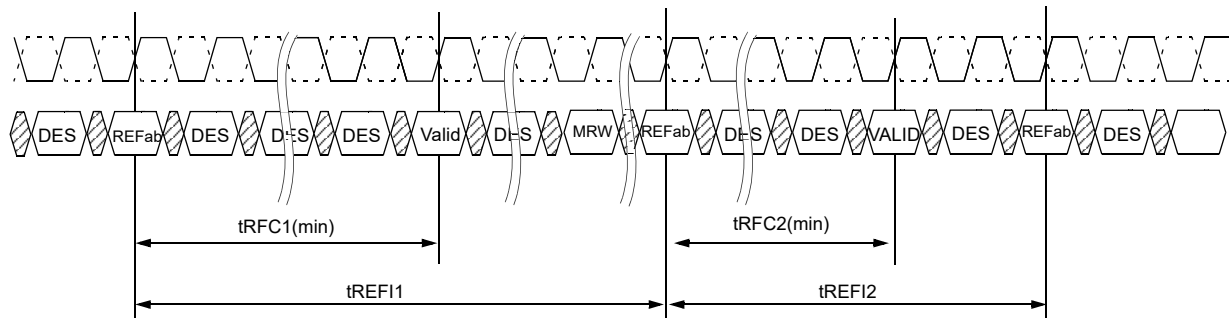
Figure 70 — Refresh Mode Change Command Timing
