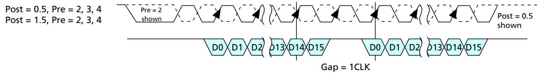
Figure 29 — Example of Consecutive Writes Operation: t_{CCD}=\text{Min}+1
