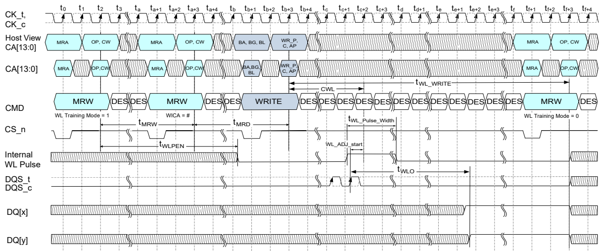
Figure 111 — Write Leveling Training Mode Timing Diagram (Internal Cycle Alignment, 2N Mode, 1 Sample)
