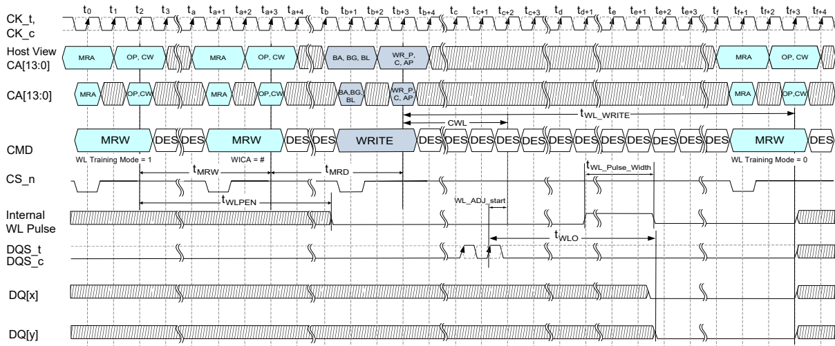
Figure 109 — Write Leveling Training Mode Timing Diagram (Internal Cycle Alignment, 2N Mode, 0 Sample)
