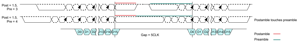
Figure 33 — Example of Consecutive Writes Operation: t_{CCD} = \text{Min} + 5
