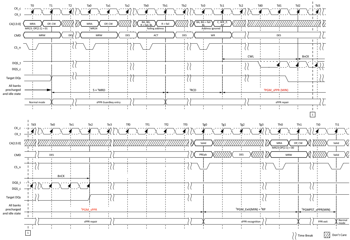
Figure 141 — sPPR Fail Row Repair
