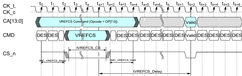
Figure 117 — Timing Diagram for VrefCS Command
