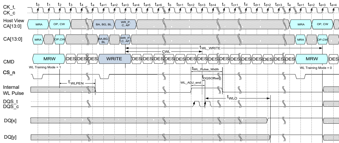
Figure 114 — Timing Diagram for final timings after Write Leveling Training is complete (2N Mode)
