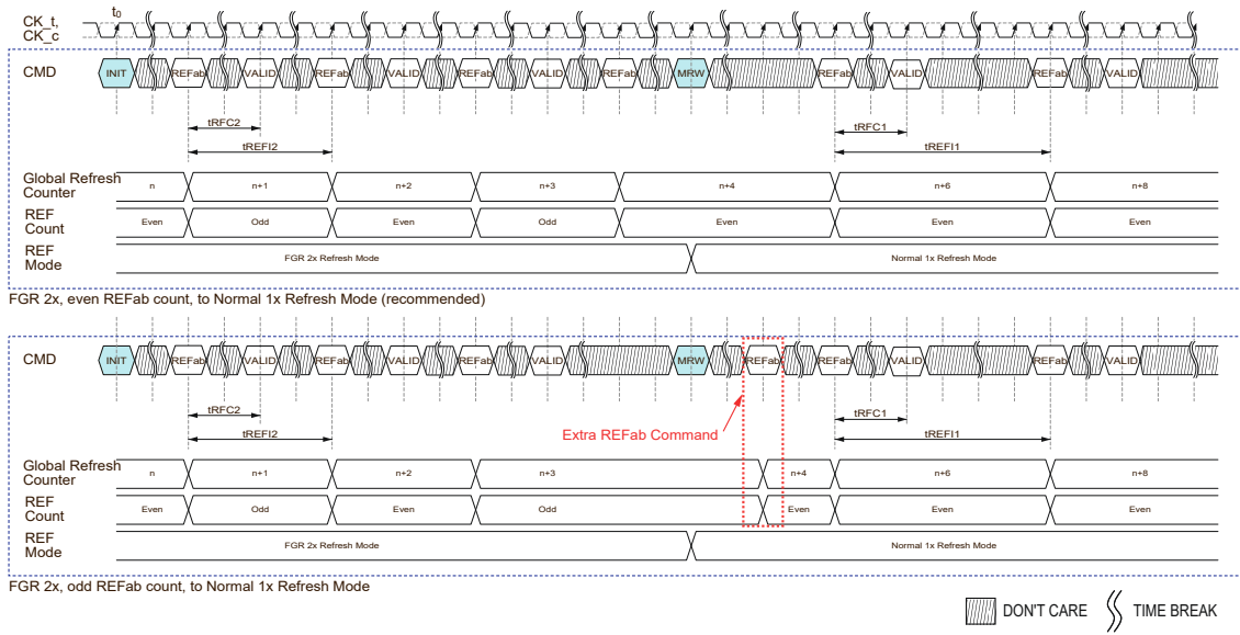
Figure 71 — Refresh Mode Change from FGR 2x to Normal 1x Command Timing
