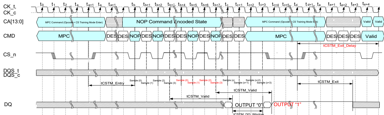
Figure 101 — Timing Diagram for CS Training Mode with Output Sample Toggle
