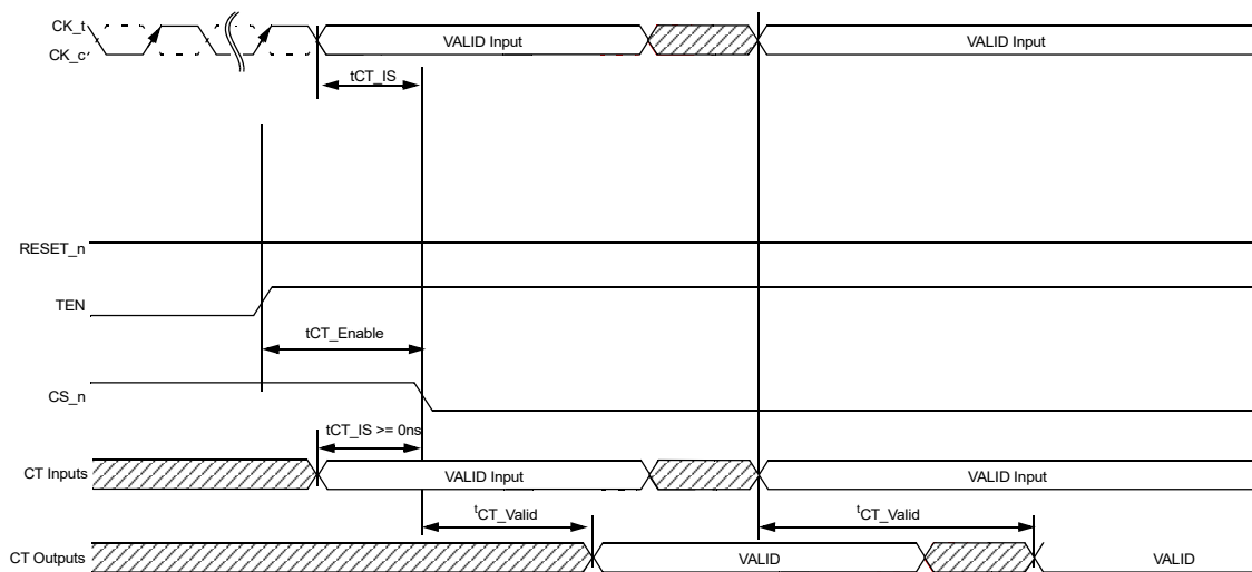
Figure 237 — Timing Diagram for Connectivity Test (CT) Mode
