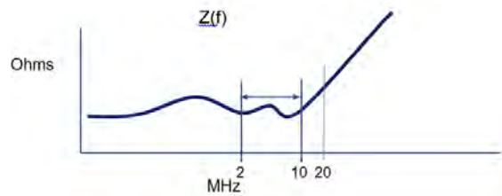
Figure 211 — Zprofile/Z(f) of the system at the DRAM package solder ball (without DRAM component)
