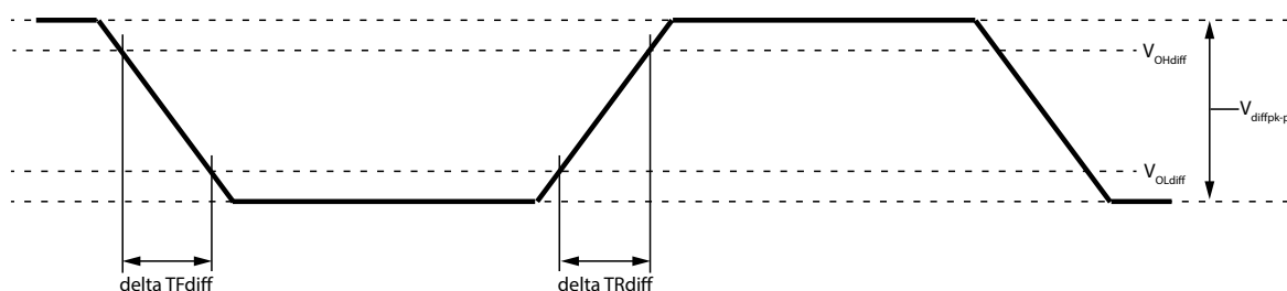
Figure 246 — Differential Output Slew Rate Definition
