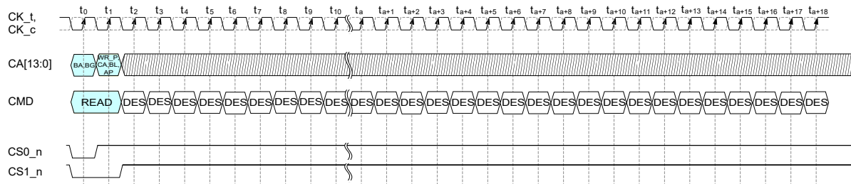
Figure 40 — Read Timing for fixed BL32 and BL32 in BL32 OTF mode
