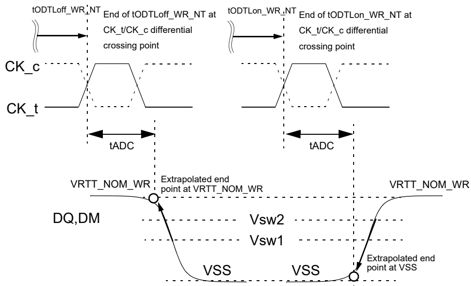
Figure 209 — tADC Measurement Method Non-Target DRAM Write
