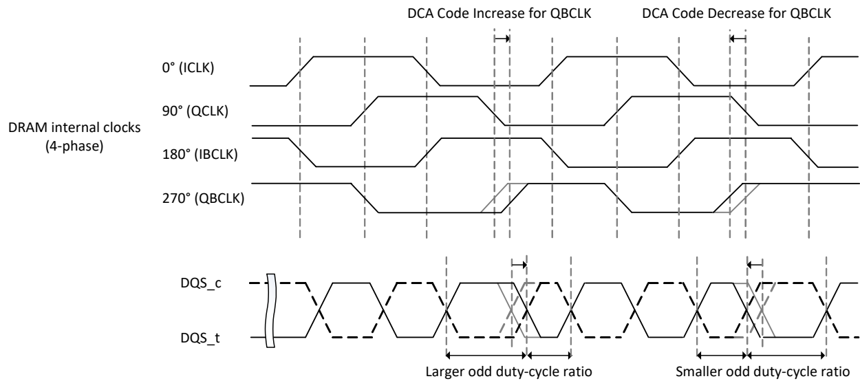
Figure 185 — Relationship between DCA Code Change for QBCLK and the 4-phase internal clocks/ DQS waveform (Example)
