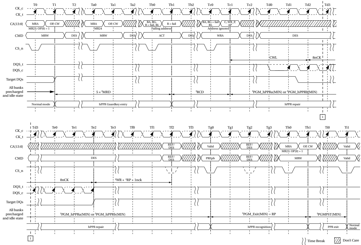
Figure 140 — hPPR Fail Row Repair
