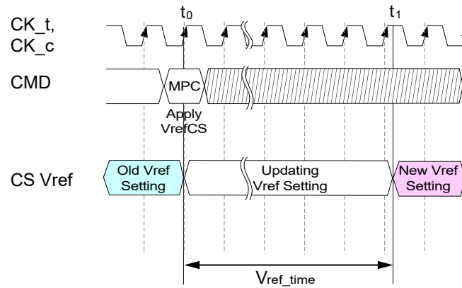
Figure 127 — Vref_time timing diagram
