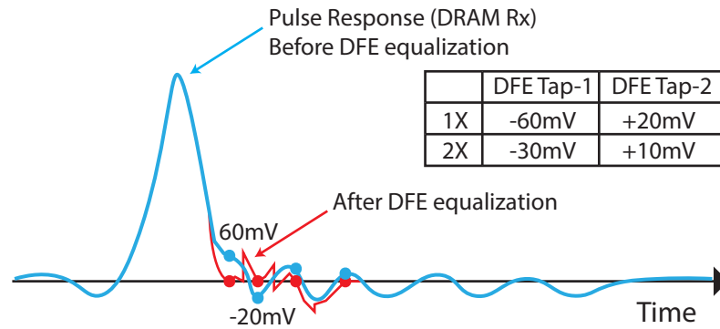
Figure 146 — Example of Pulse Response of a Reflective Channel
