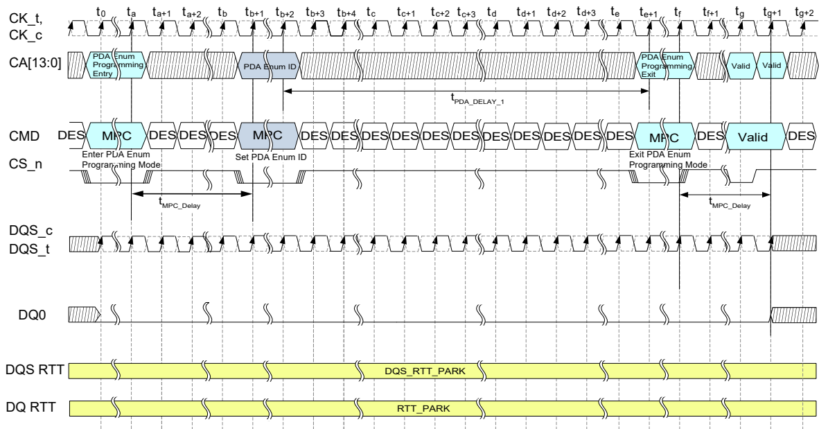
Figure 81 — Single Device PDA Enumerate Programming in Continuous DQS Toggle Mode
