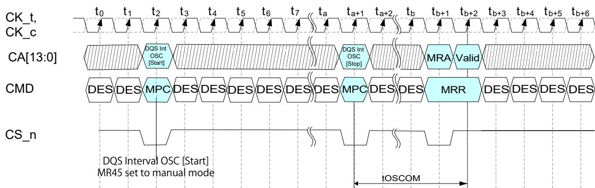
Figure 153 — DQS Interval Oscillator Manual Mode Timing Diagram
