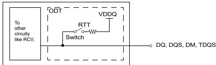
Figure 188 — Functional Representation of ODT
