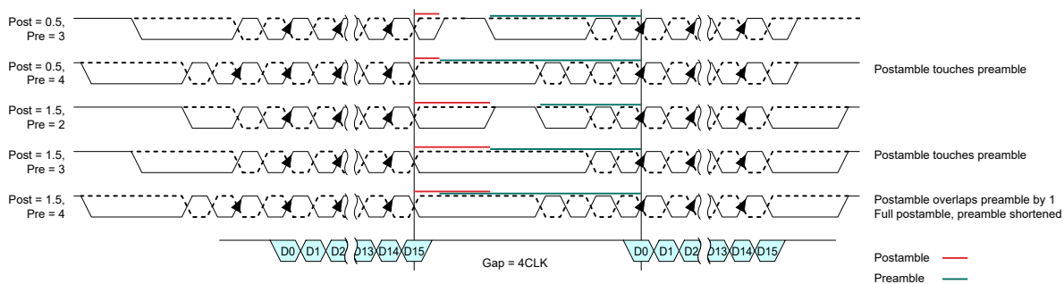
Figure 32 — Example of Consecutive Writes Operation: t_{CCD} = \text{Min} + 4
