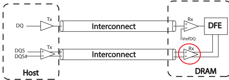
Figure 229 — Example of DDR5 Memory Interconnect
