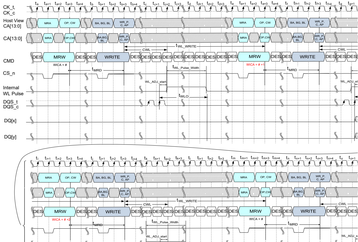
Figure 113 — Consecutive Write commands during Write Leveling Training Mode Example (Internal Training, 2N Mode, 4 Samples)
