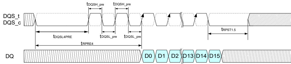
Figure 19 — DQS Timing While 4tCK Read Preamble and 1.5tCK Postamble
