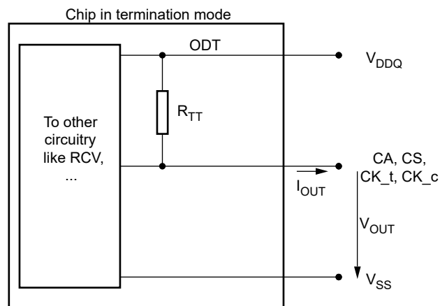
Figure 205 — A functional representation of the on-die termination
