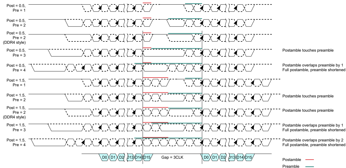
Figure 25 — Example of Consecutive Reads Operation: t_{CCD} = \text{Min} + 3
