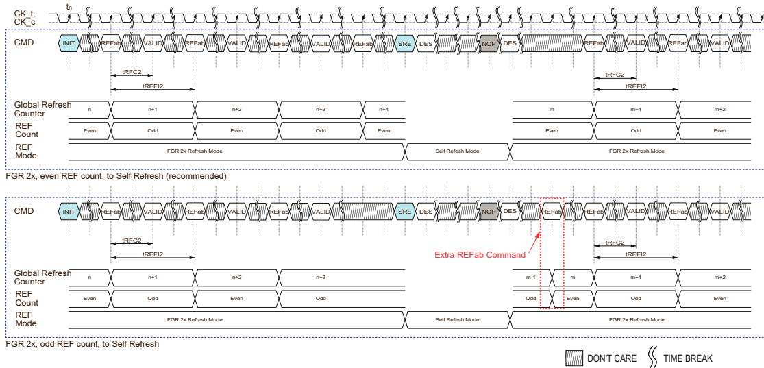
Figure 75 — FGR 2x to SREF Command Timing
