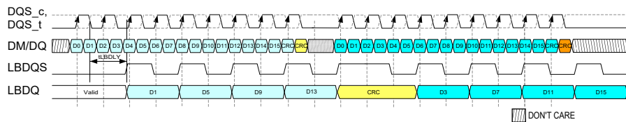
Figure 174 — Loopback Normal Output Mode 4-Way PhaseB with CRC, 1CK Gap Example
