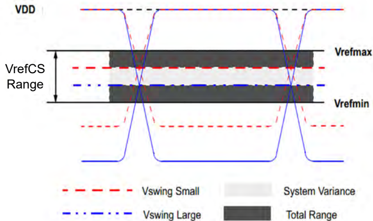
Figure 125 — VrefCS operating range(Vrefmin, Vrefmax)
