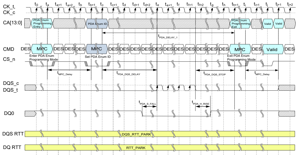
Figure 80 — Single Device PDA Enumerate Programming in Legacy Mode
