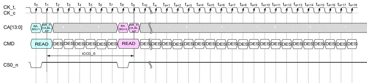
Figure 41 — Read Timings for BL16 in BL32 OTF mode
