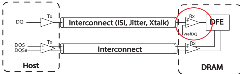
Figure 235 — Example of Rx Stressed Test Setup in the Presence of ISI, Jitter and Crosstalk
