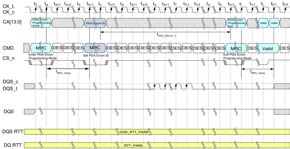
Figure 85 — Single Device PDA Enumerate Programming “Don’t enumerate” Case in Legacy Mode.
