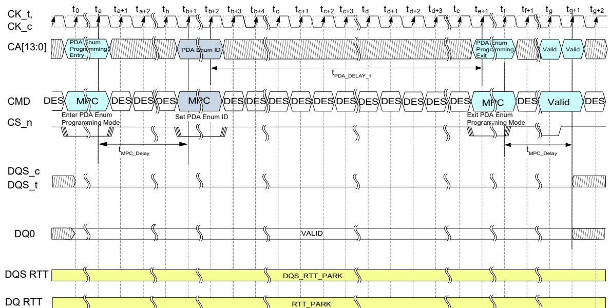
Figure 88 — Single Device PDA Enumerate Programming “Don’t Enumerate” Case for DQ is VALID and DQS is Differentially LOW
