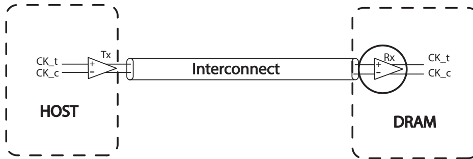
Figure 224 — HOST driving clock signals to the DRAM
