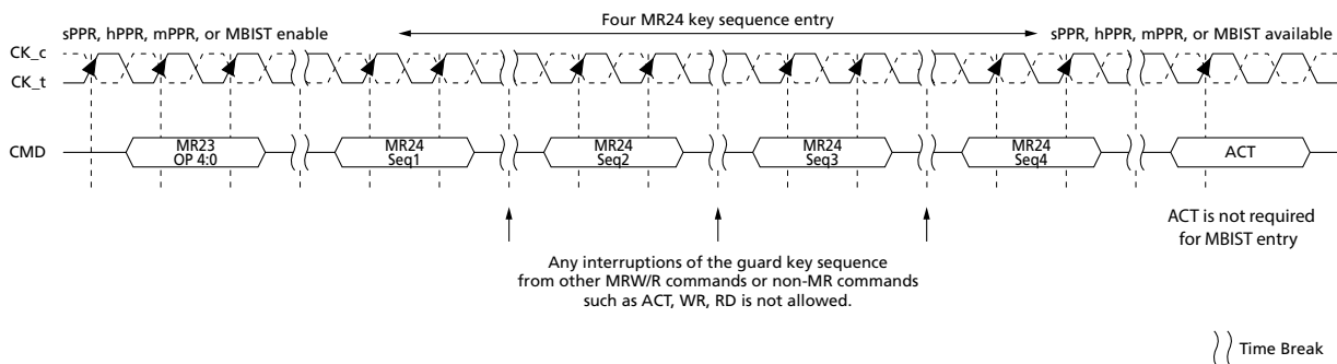
Figure 139 — Guard Key Timing Diagram
