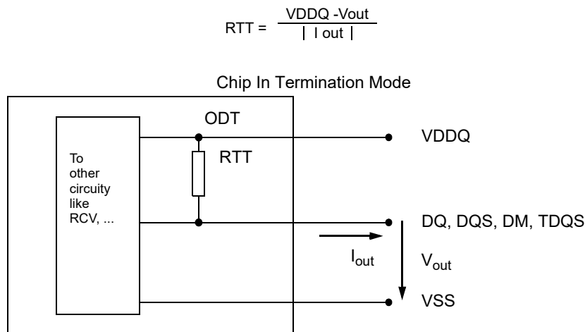
Figure 189 — On Die Termination
