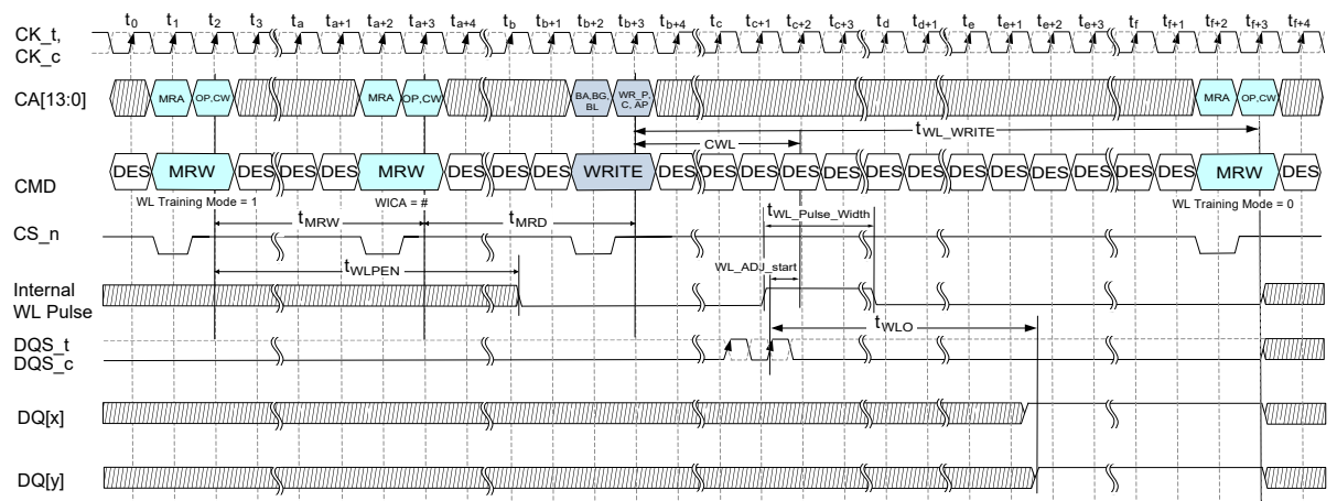
Figure 112 — Write Leveling Training Mode Timing Diagram (Internal Cycle Alignment, 1N Mode, 1 Sample)
