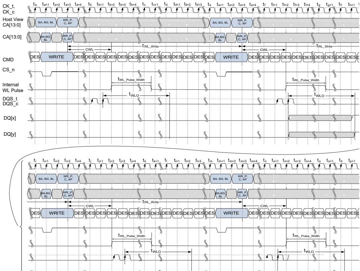
Figure 107 — Consecutive Write commands during Write Leveling Training Mode Example (External Training, 2N Mode, 4 Samples)
