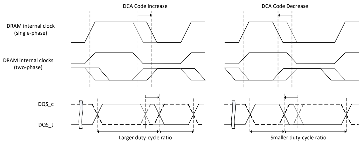
Figure 182 — Relationship between DCA code Change and the single/two-phase internal clock(s)/ DQS waveform (Example)
