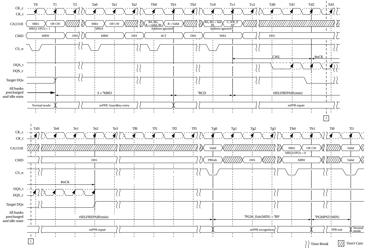
Figure 143 — mPPR Row Repair
