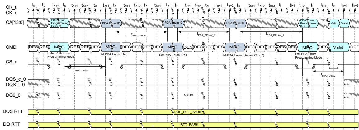
Figure 92 — Multi Device PDA Enumerate Programming “Don’t Enumerate” Case for VALID DQ and Differentially Low DQS
