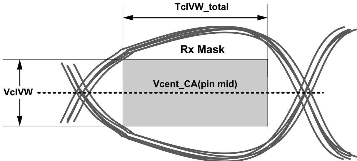
Figure 219 — CA Receiver (Rx) mask
