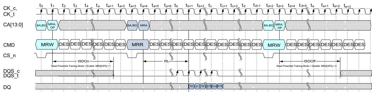
Figure 98 — Timing Diagram for Read Preamble Training Mode Entry, Read Training Pattern Access and Read Preamble Training Mode Exit
