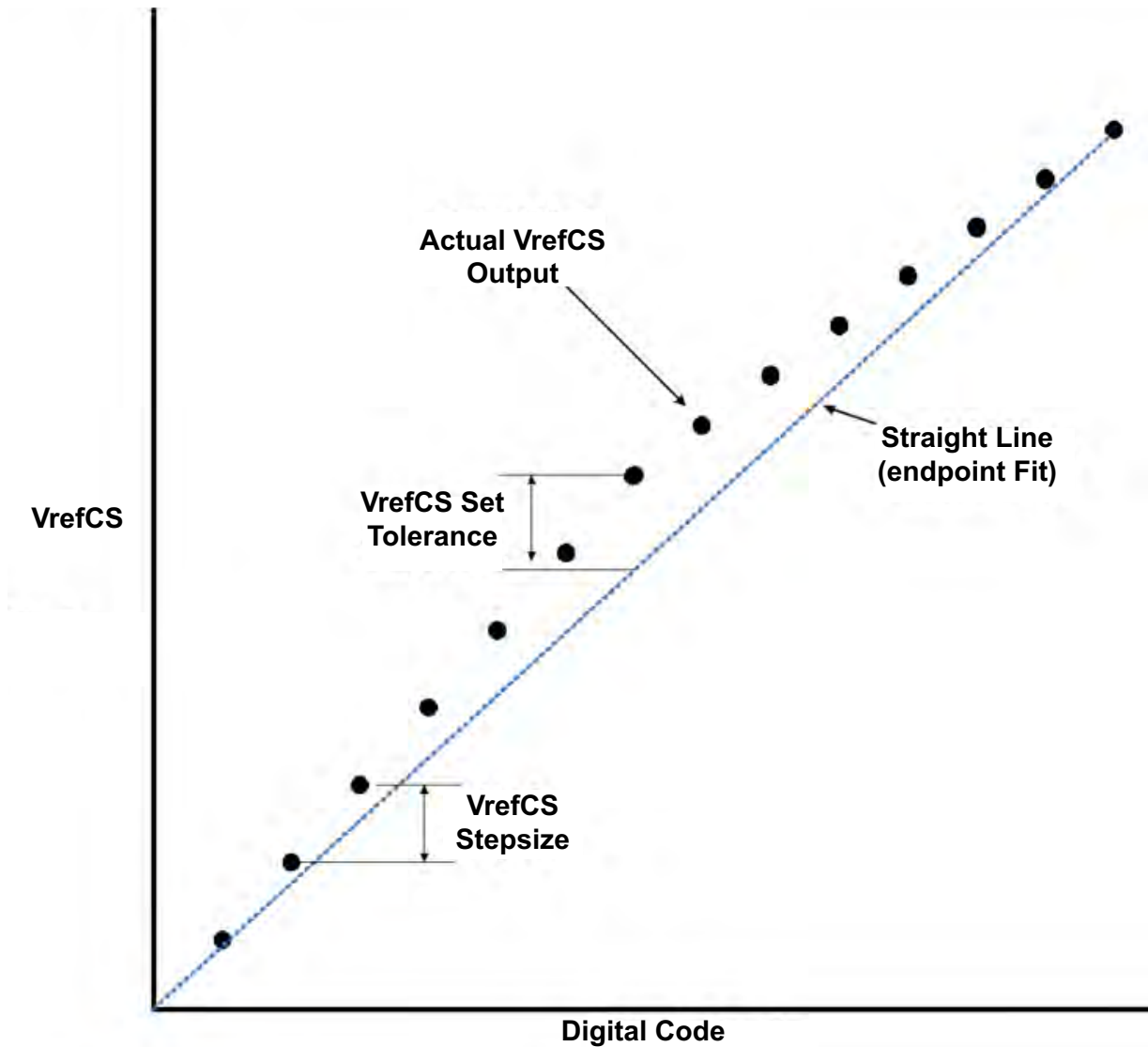
Figure 126 — Example of Vref set tolerance (max case only shown) and stepsize
