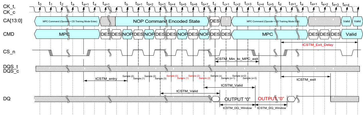
Figure 100 — Timing Diagram for CS Training Mode with Consecutive Output Samples = 0
