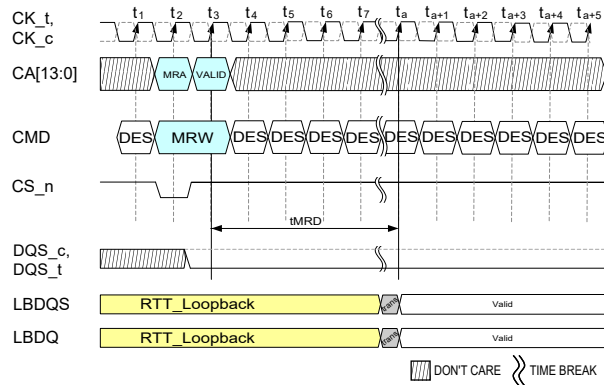
Figure 168 — Loopback Normal Output Mode Entry
