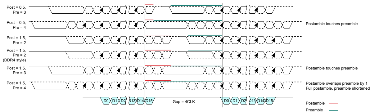
Figure 26 — Example of Consecutive Reads Operation: t_{CCD} = \text{Min} + 4
