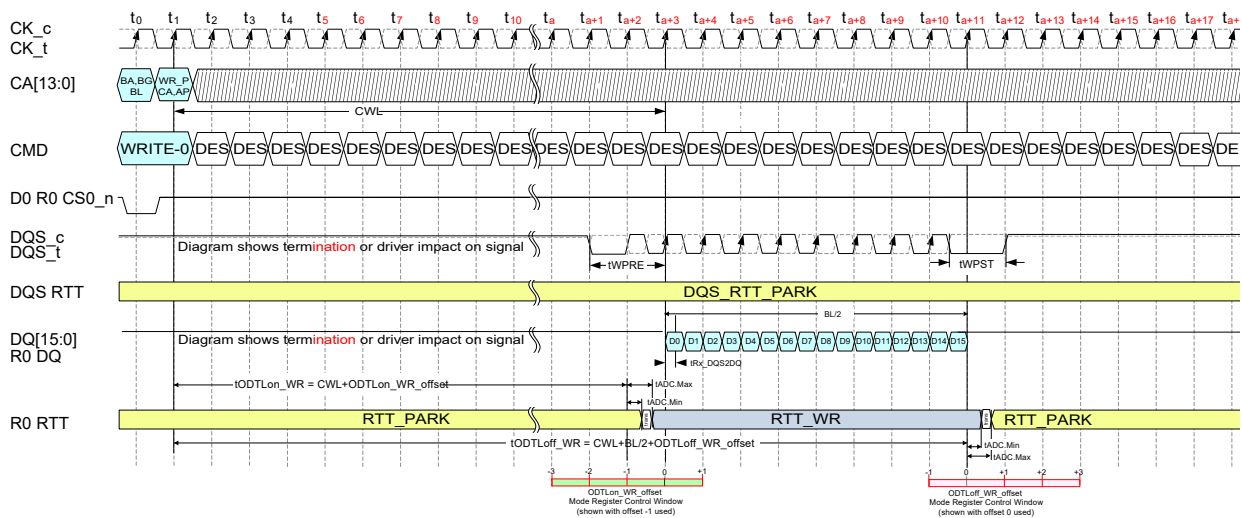
Figure 192 — Example 1 of Burst Write Operation ODT Latencies and Control Diagrams
