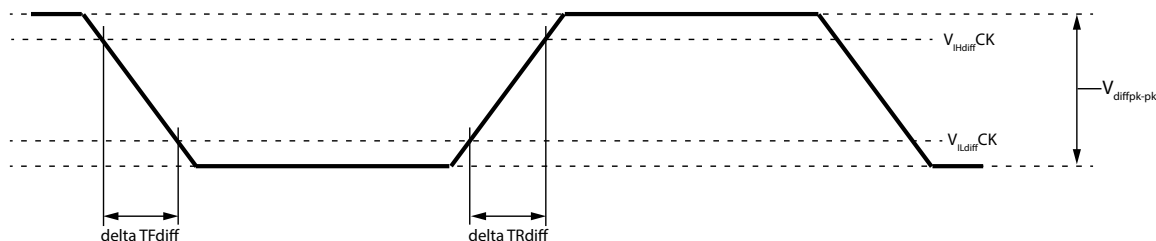
Figure 227 — Differential Input Slew Rate Definition for CK_t, CK_c
