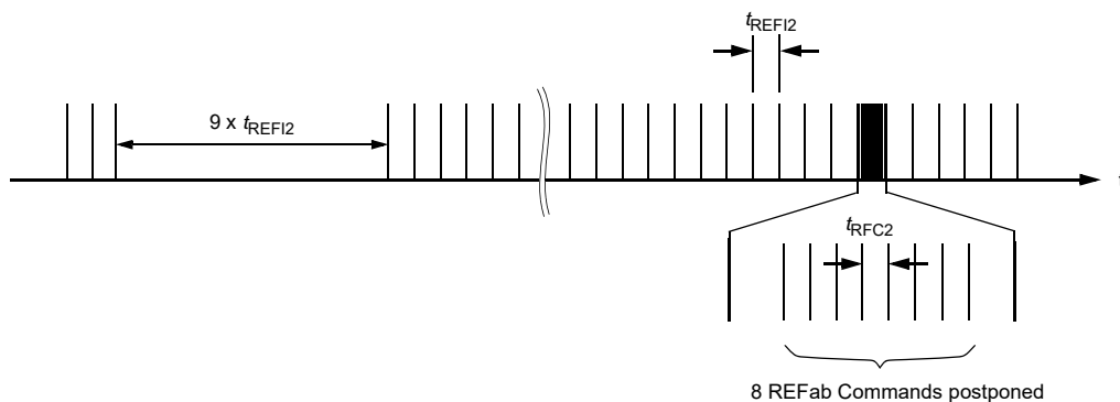
Figure 74 — Postponing Refresh Commands (Example of Fine Granularity Refresh Mode - t_{REFI2} , t_{RFC2} )
