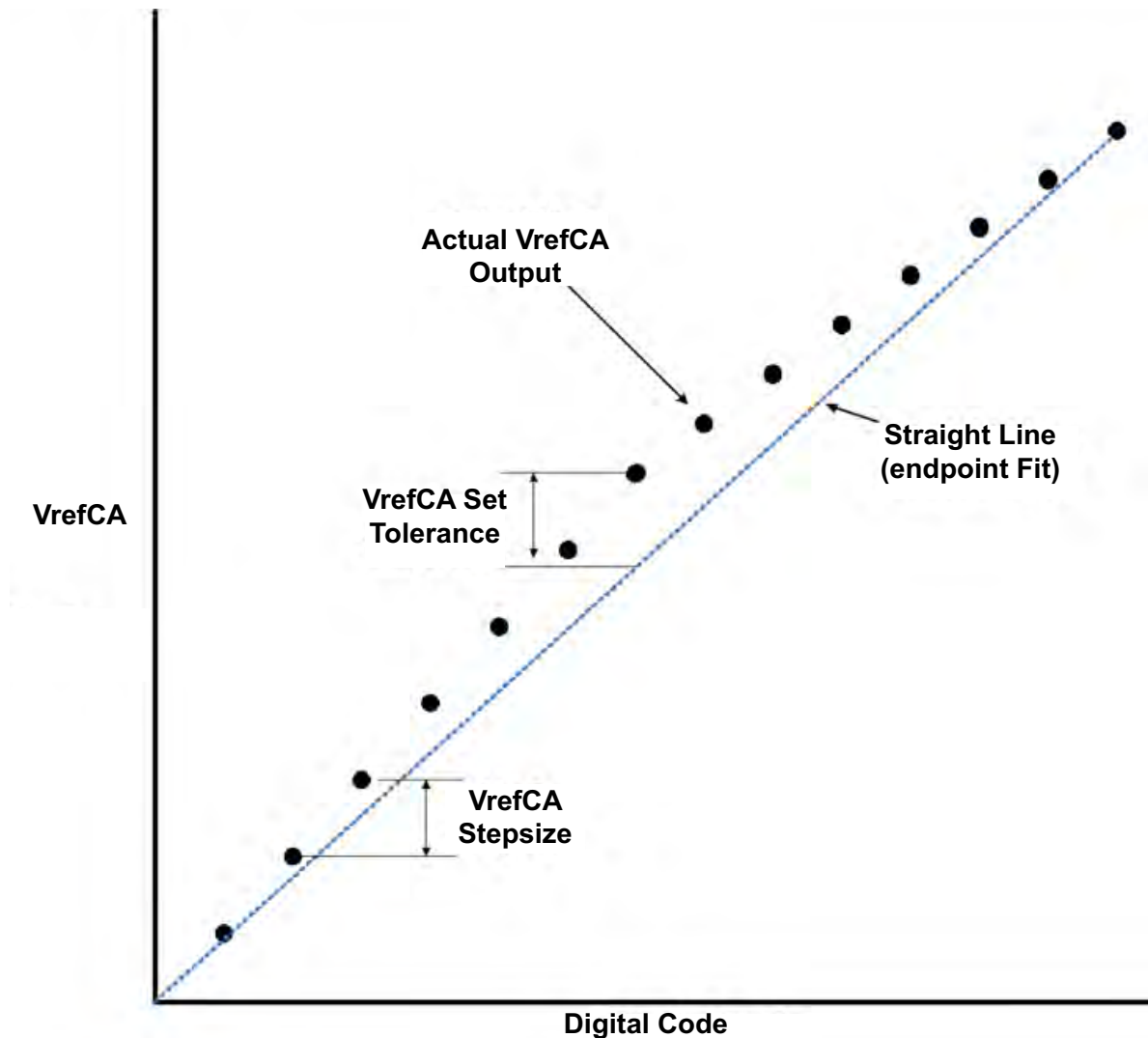
Figure 119 — Example of Vref set tolerance (max case only shown) and stepsize
