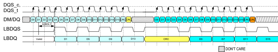
Figure 175 — Loopback Normal Output Mode 4-Way PhaseB with CRC, 2 CK Gap Example
