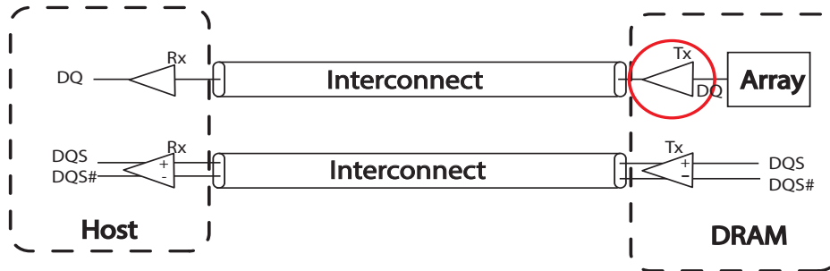
Figure 247 — Example of DDR5 Memory Interconnect
