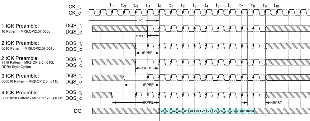
Figure 12 — Example of Read Preamble Modes (default) & w/1.5 tCK Postamble
