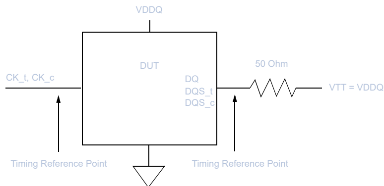
Figure 252 — Reference Load for AC Timing and Output Slew Rate
