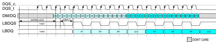
Figure 177 — Loopback Write Burst Output Mode 4-Way PhaseC WPRE=2CK Example
