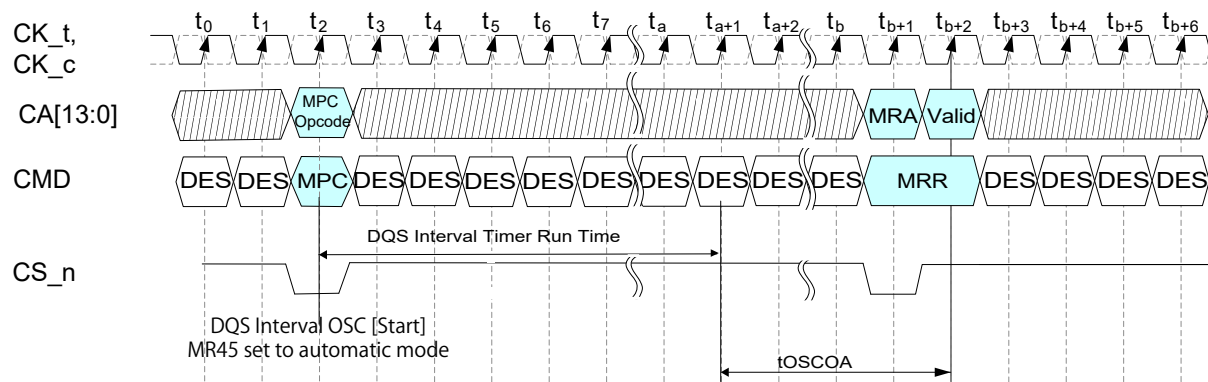
Figure 154 — DQS Interval Oscillator Automatic Mode Timing Diagram
