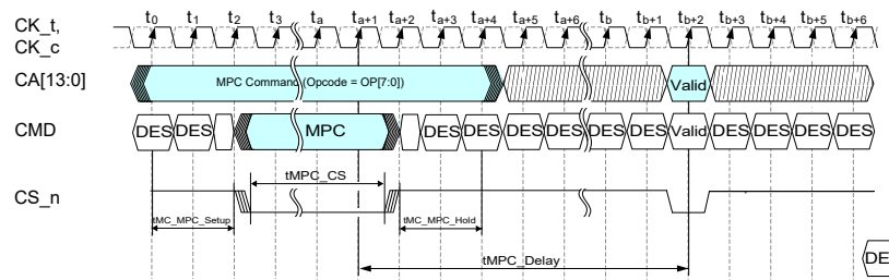
Figure 78 — MPC Function Timing to 1-Cycle Command
