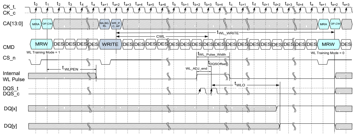
Figure 115 — Timing Diagram for final timings after Write Leveling Training is complete (1N Mode)
