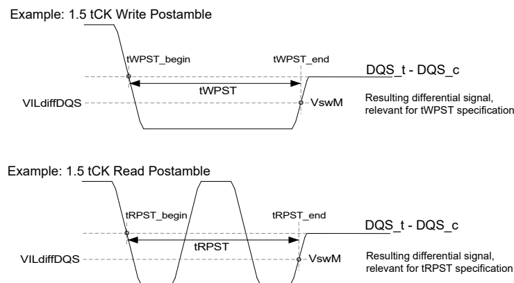
Figure 21 — Method for measuring Postamble start and end points
