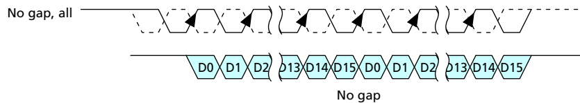
Figure 22 — Example of Seamless Reads Operation: tCCD=Min
