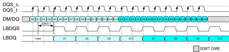
Figure 169 — Loopback Normal Output 4-Way Mode PhaseB Example
