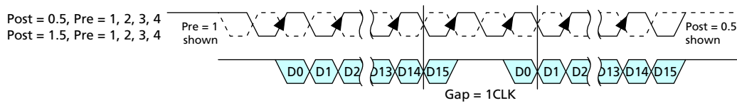
Figure 23 — Example of Consecutive Reads Operation: tCCD=Min+1
