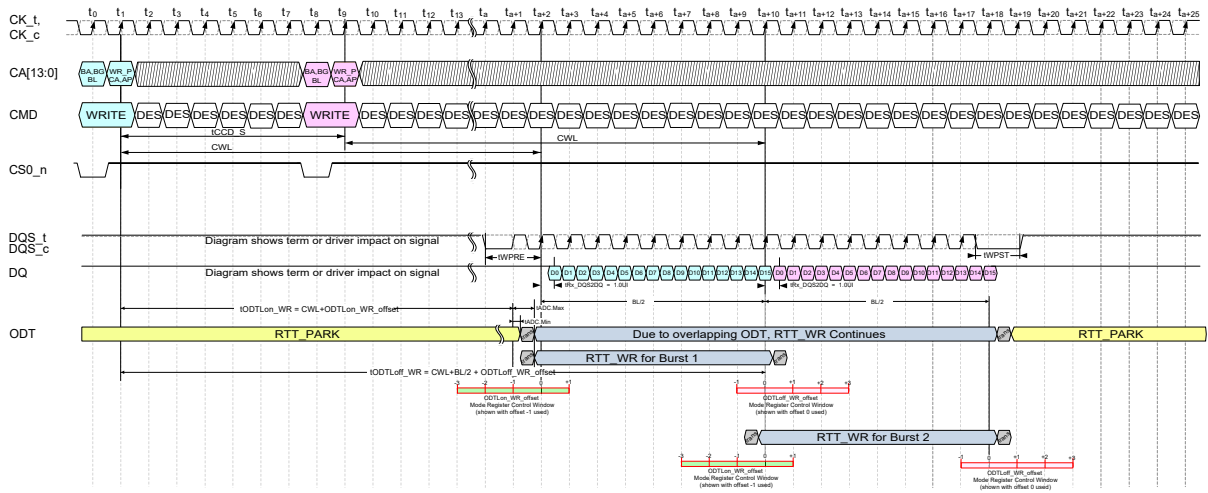
Figure 197 — WRITE (BL16) to WRITE (BL16), Different Bank, Seamless Bursts
