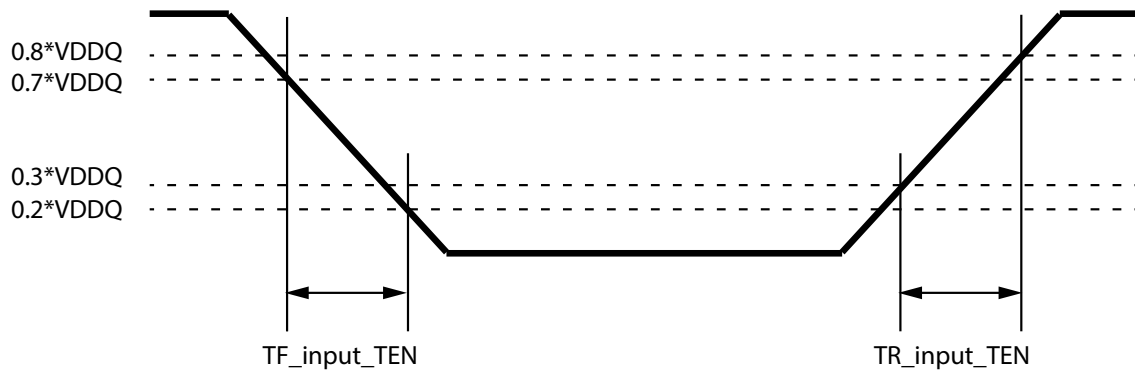
Figure 238 — TEN Input Slew Rate Definition
