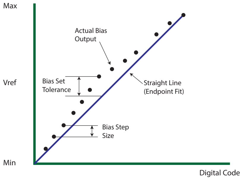
Figure 148 — Example of to be revised for INL/DNL
