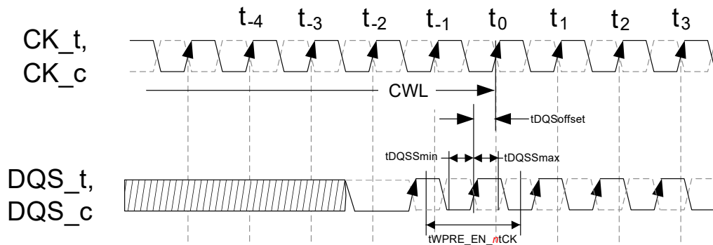
Figure 59 — tDQSS : DRAM external CLK-to-DQS Variation
