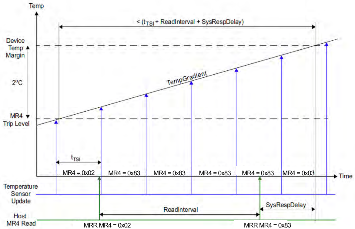
Figure 77 — Temp Sensor Timing Diagram
