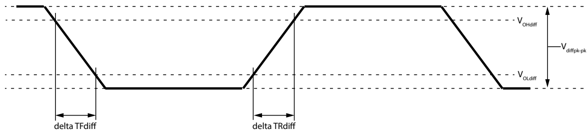
Figure 245 — Differential Output Slew Rate Definition
