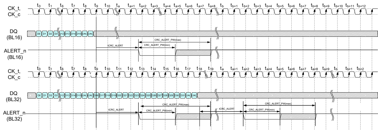
Figure 163 — CRC Error Reporting Timing diagram
