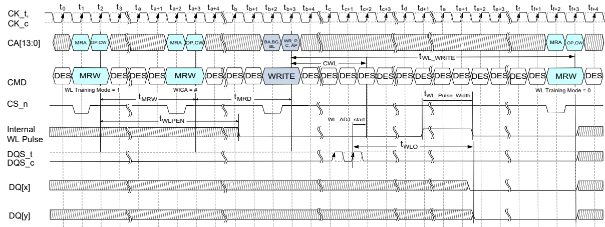
Figure 110 — Write Leveling Training Mode Timing Diagram (Internal Cycle Alignment, 1N Mode, 0 Sample)
