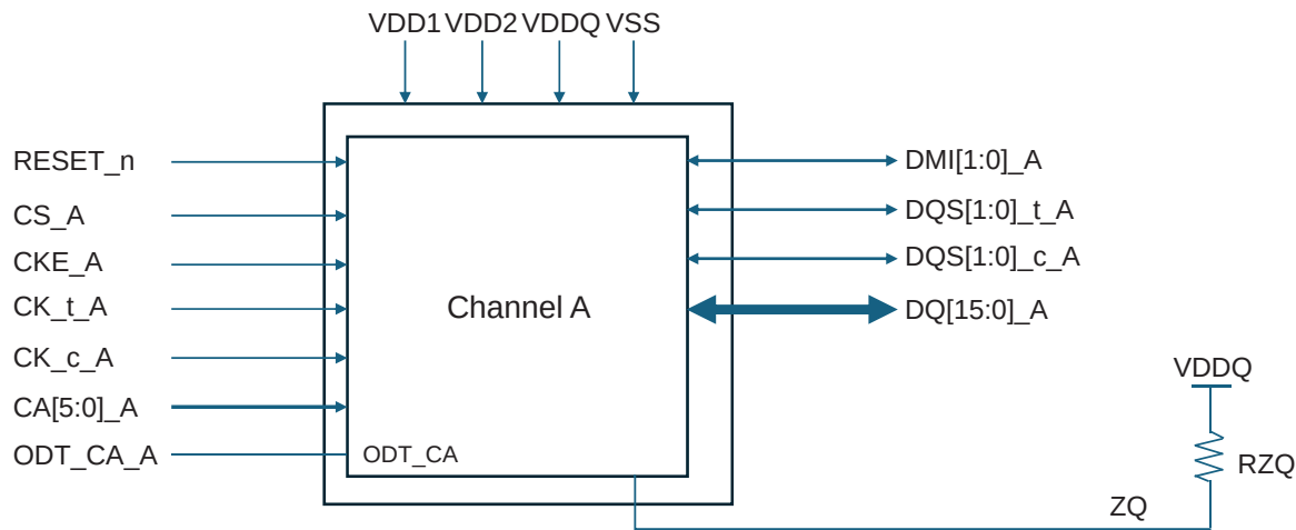
Figure 3.1 – Single-channel (x16) Package Diagram
