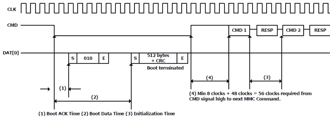
[Figure 23] e-NAND state diagram (Boot mode)
