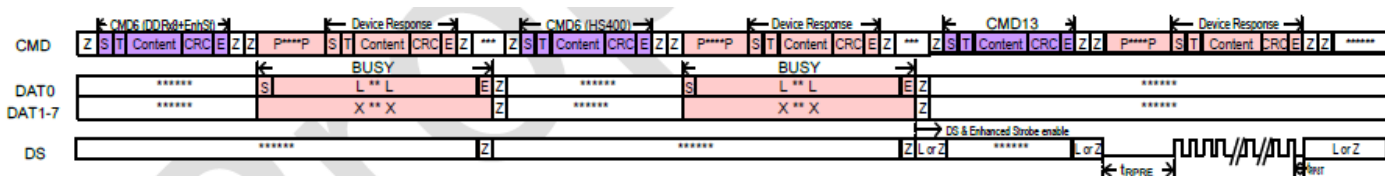
[Figure 13] HS400 mode change with Enhanced Strobe
