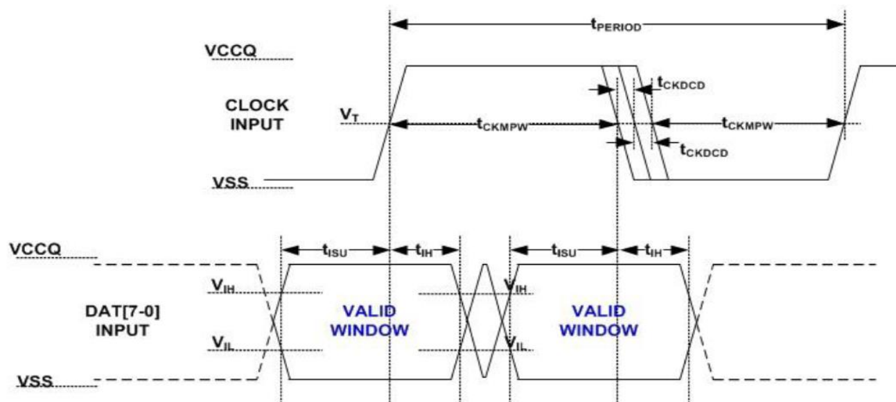
[Figure 4] HS400 Device input timing
