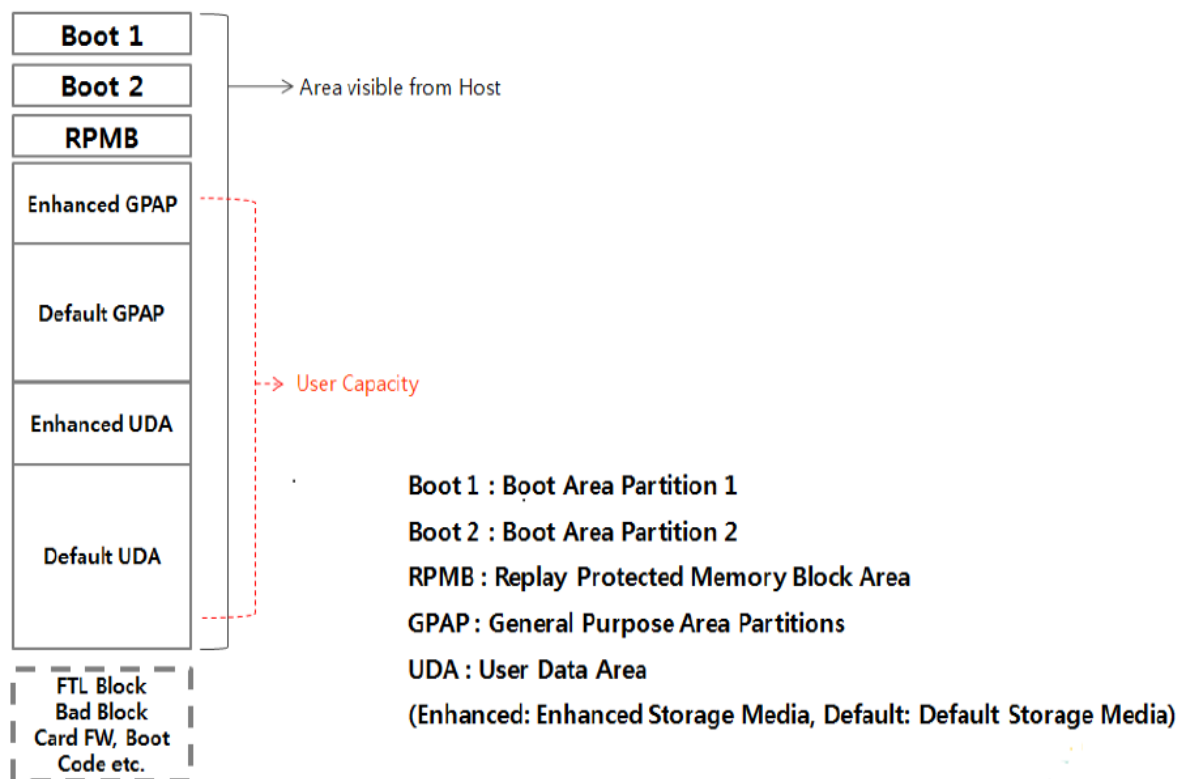
[Figure 22] Partition diagram
