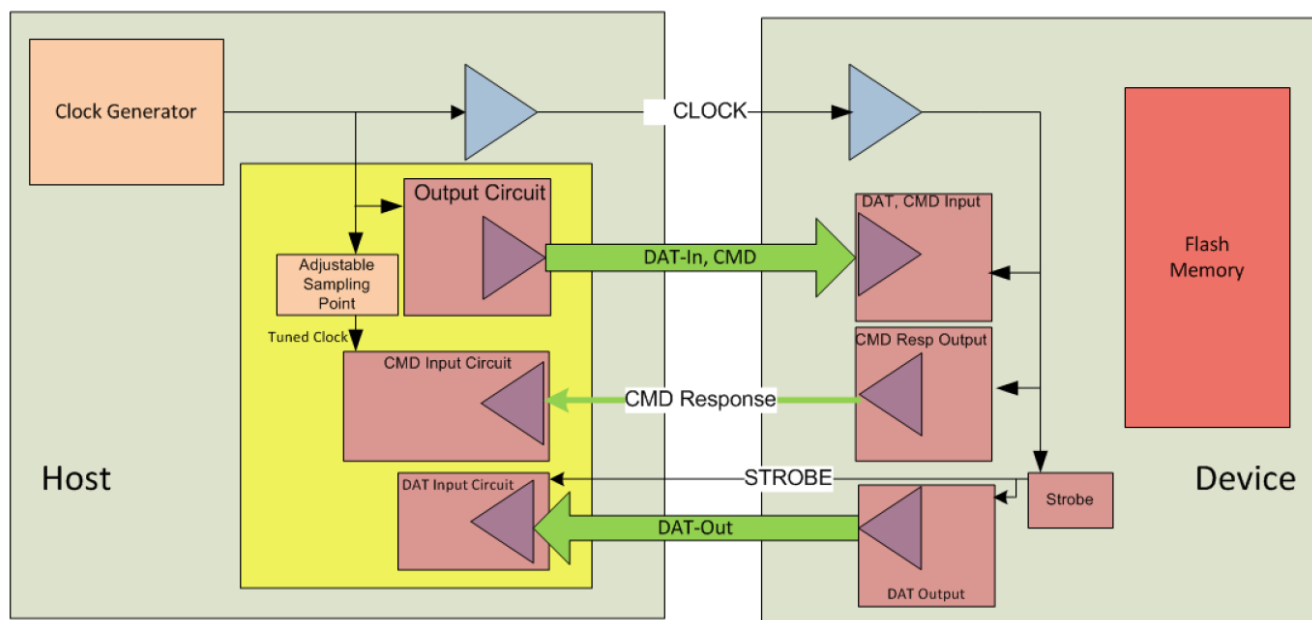
[Figure 6] HS400 Host and Device block diagram
