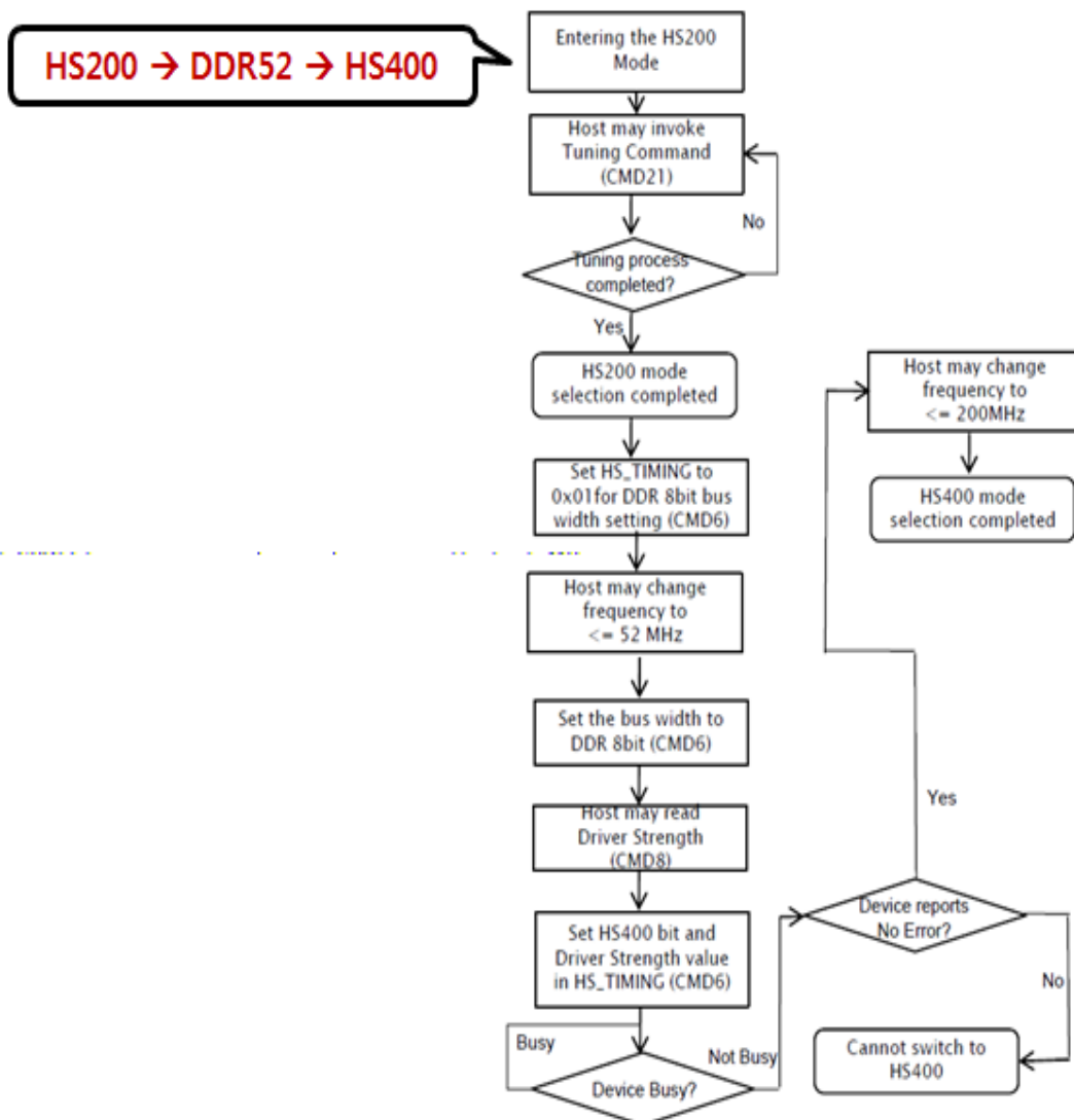
[Figure 7] HS400 Bus mode selection sequence
