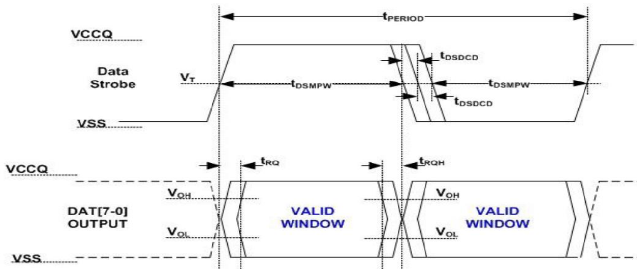
[Figure 5] HS400 Device output timing
