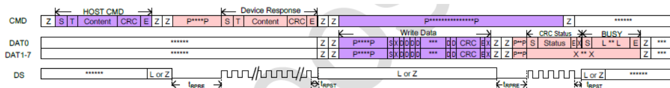
[Figure 12] Enhanced Strobe signals for CMD Response and CRC Response (Write operation)
