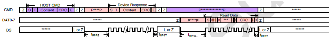
[Figure 11] Enhanced Strobe signals for CMD Response and Data Out (Read operation)
