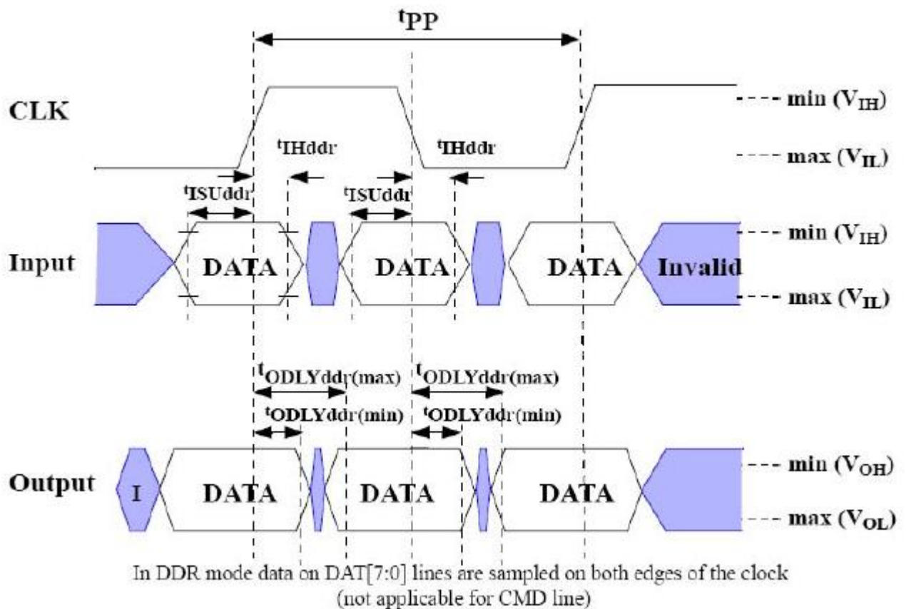
[Figure 16] Timing diagram : data input/output in dual rate mode
