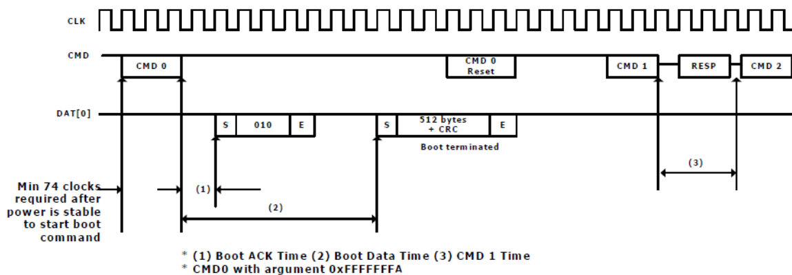
[Figure 24] e-NAND state diagram (Alternative boot mode)
