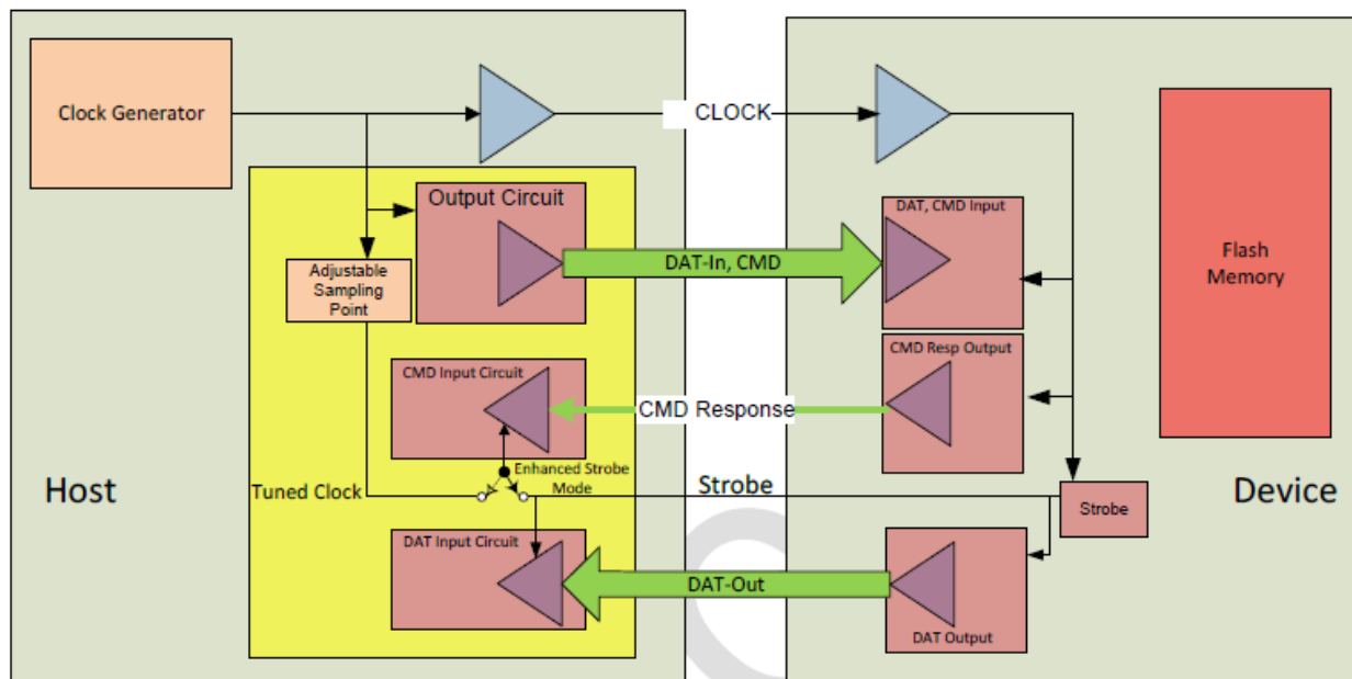
[Figure 10] HS400 Host and Device block diagram (when Enhanced Strobe is enabled)
