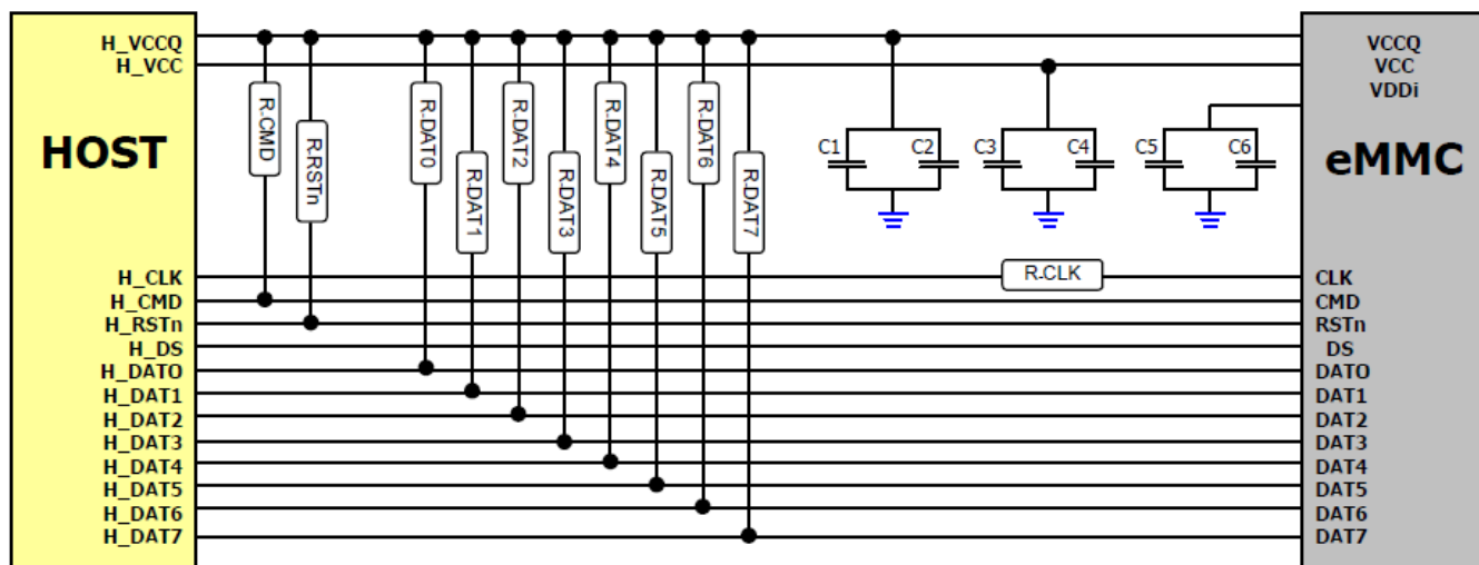
[Figure 21] Connection guide drawing
