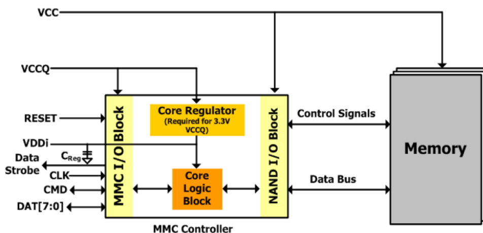
[Figure 20] e-NAND internal power diagram
