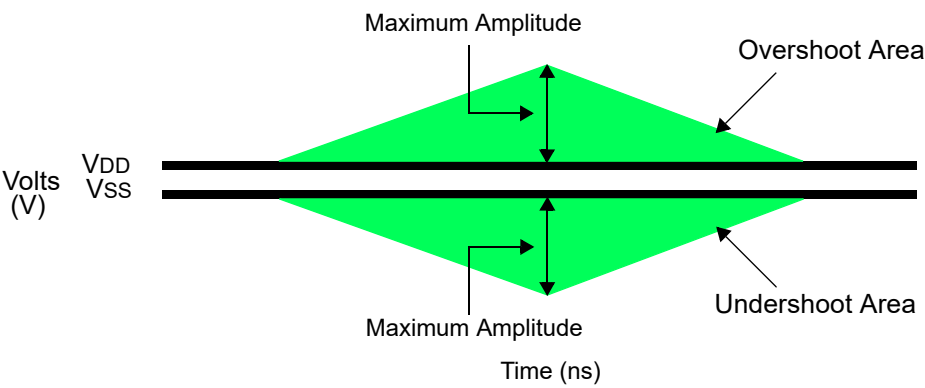
Figure 5. AC Overshoot and Undershoot Definition for Address and Control Pins
